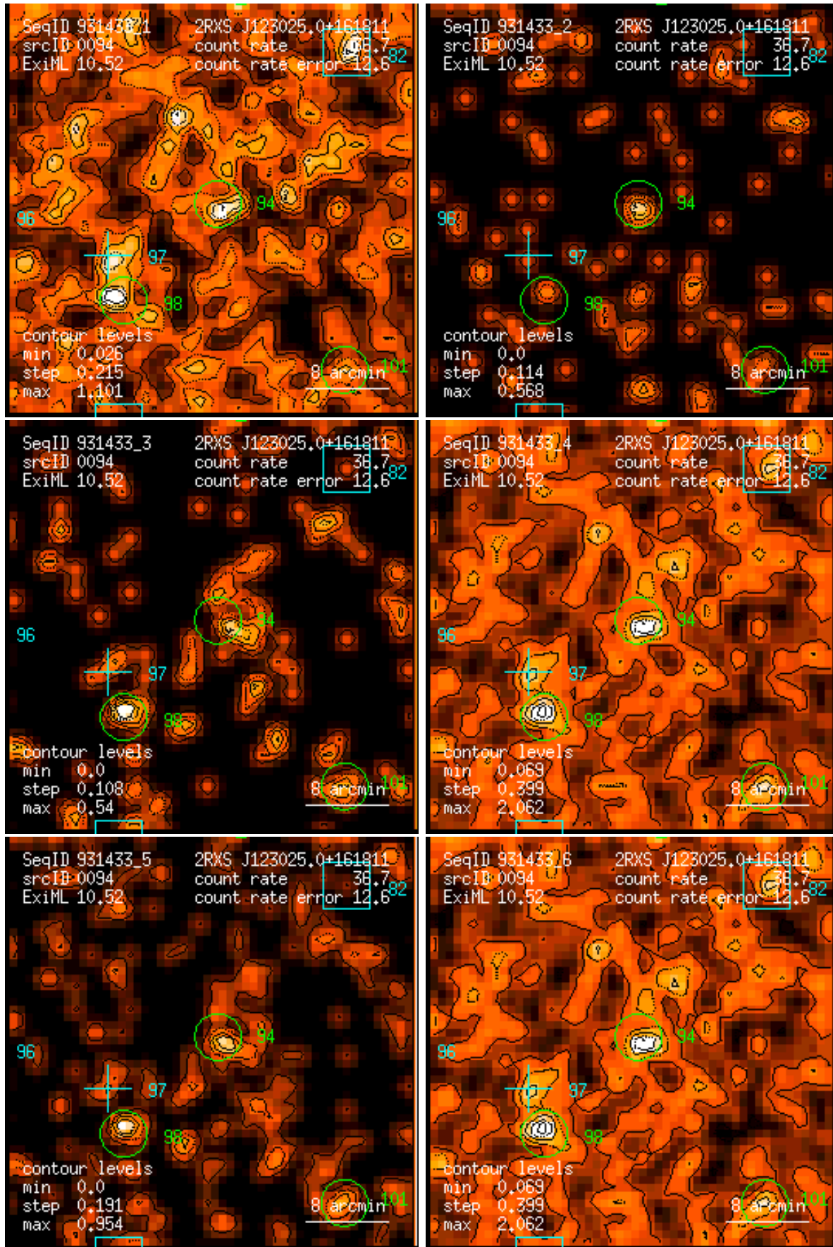
Figure 94: RASS 931433: detection 0094: band rate images, Gaussian filter: (1) PSPC channels 11 – 41, (2) 52 – 90, (3) 91 – 201, (4) 11 – 235, (5) 52 – 201, (6) 11 – 201. Broad band rates in counts/ks. Band rate contour levels in counts/ks/arcmin 2 .
