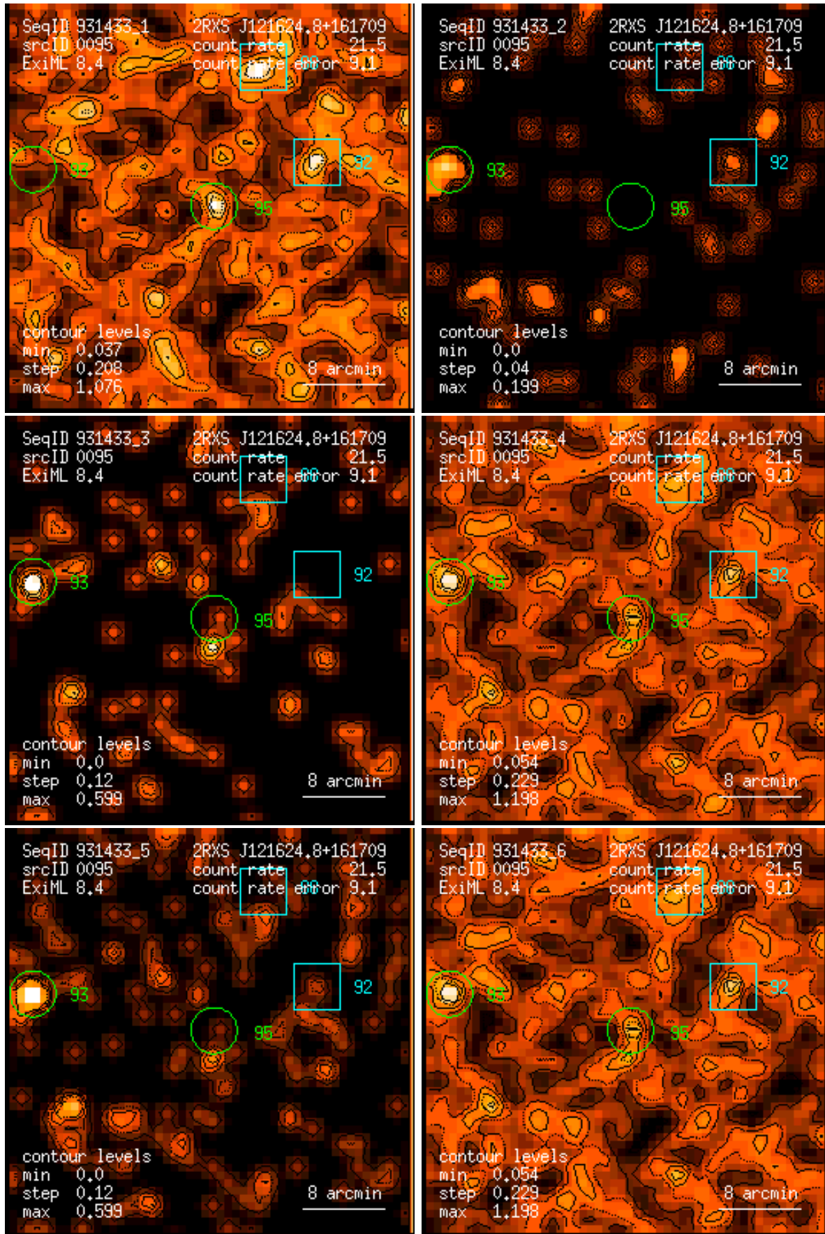
Figure 95: RASS 931433: detection 0095: band rate images, Gaussian filter: (1) PSPC channels 11 – 41, (2) 52 – 90, (3) 91 – 201, (4) 11 – 235, (5) 52 – 201, (6) 11 – 201. Broad band rates in counts/ks. Band rate contour levels in counts/ks/arcmin 2 .
