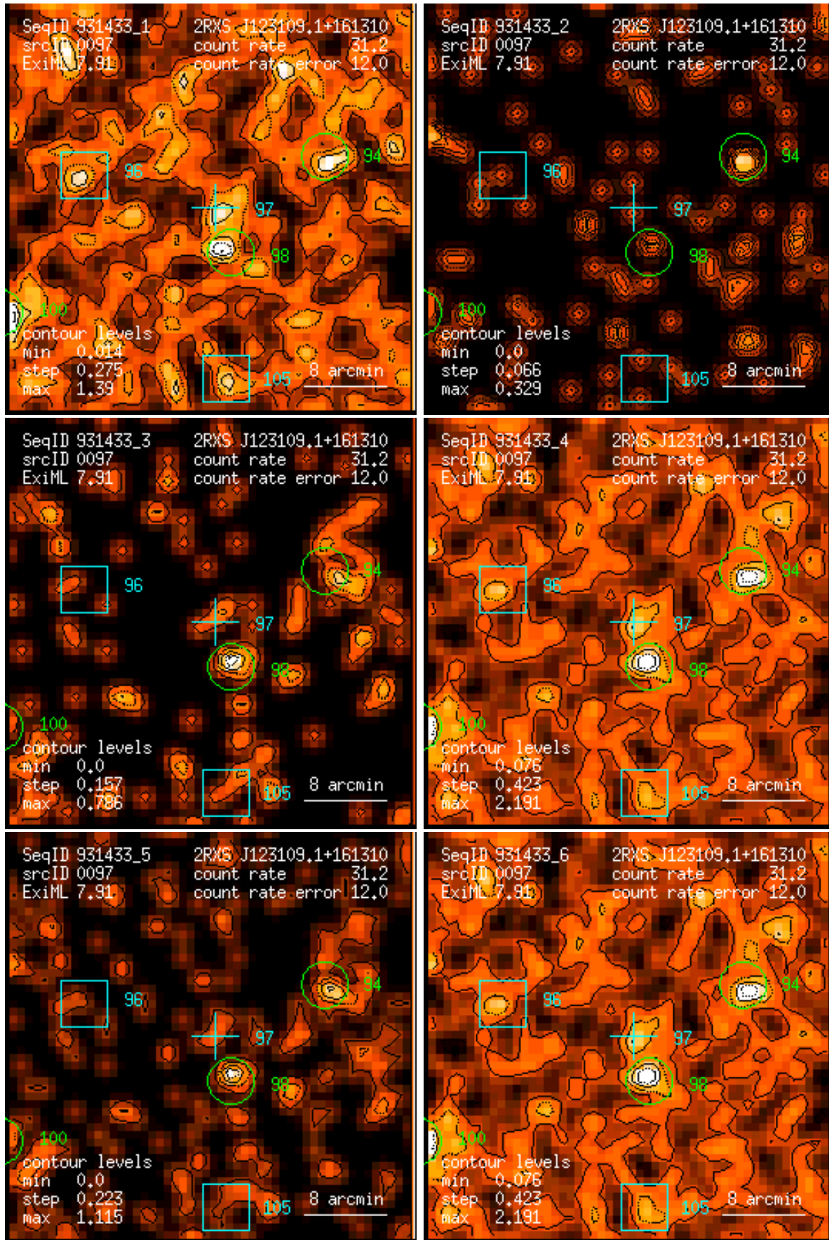
Figure 97: RASS 931433: detection 0097: band rate images, Gaussian filter: (1) PSPC channels 11 – 41, (2) 52 – 90, (3) 91 – 201, (4) 11 – 235, (5) 52 – 201, (6) 11 – 201. Broad band rates in counts/ks. Band rate contour levels in counts/ks/arcmin 2 .
