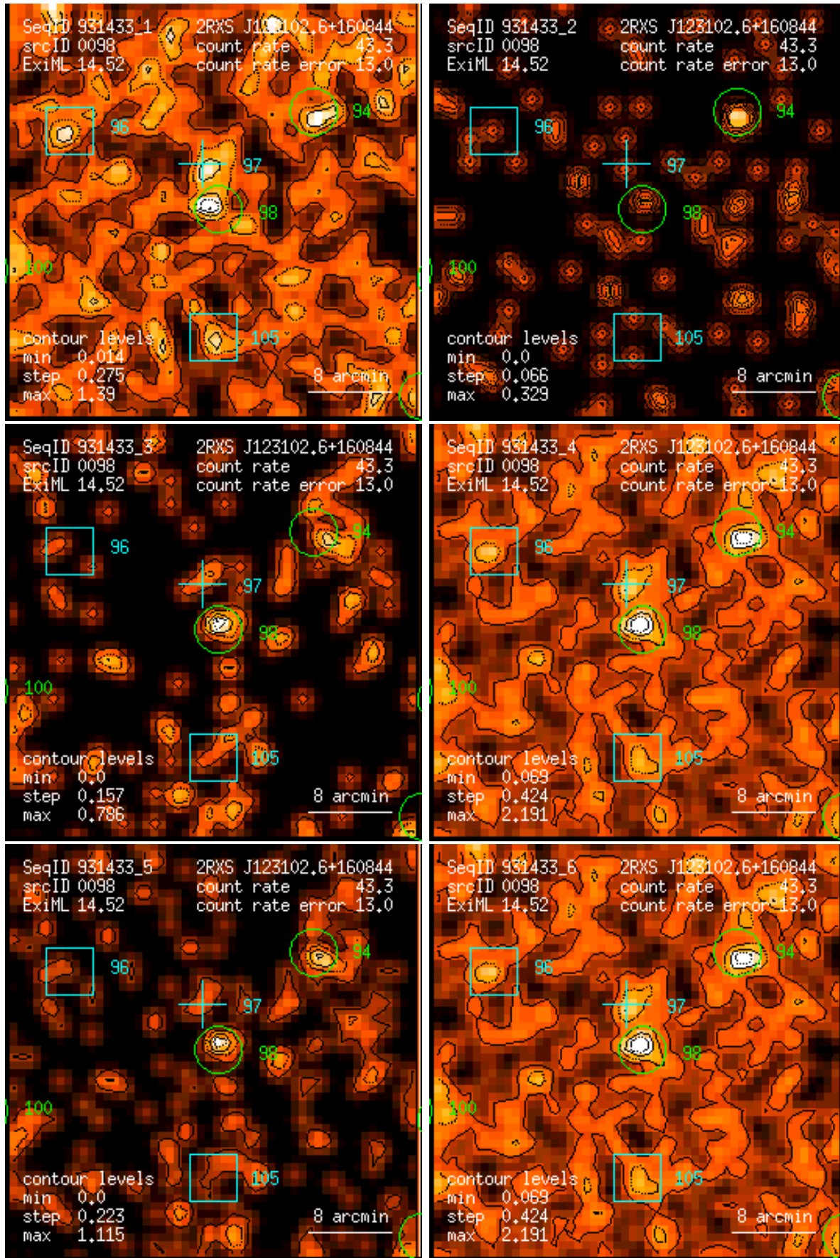
Figure 98: RASS 931433: detection 0098: band rate images, Gaussian filter: (1) PSPC channels 11 – 41, (2) 52 – 90, (3) 91 – 201, (4) 11 – 235, (5) 52 – 201, (6) 11 – 201. Broad band rates in counts/ks. Band rate contour levels in counts/ks/arcmin 2 .
