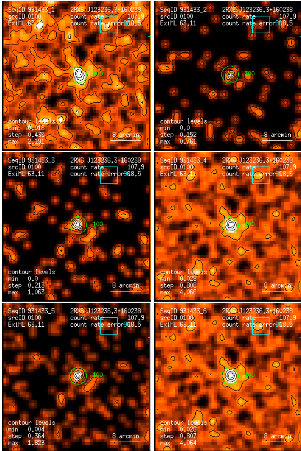
Figure 100: RASS 931433: detection 0100: band rate images, Gaussian filter: (1) PSPC channels 11 – 41, (2) 52 – 90, (3) 91 – 201, (4) 11 – 235, (5) 52 – 201, (6) 11 – 201. Broad band rates in counts/ks. Band rate contour levels in counts/ks/arcmin 2 .
