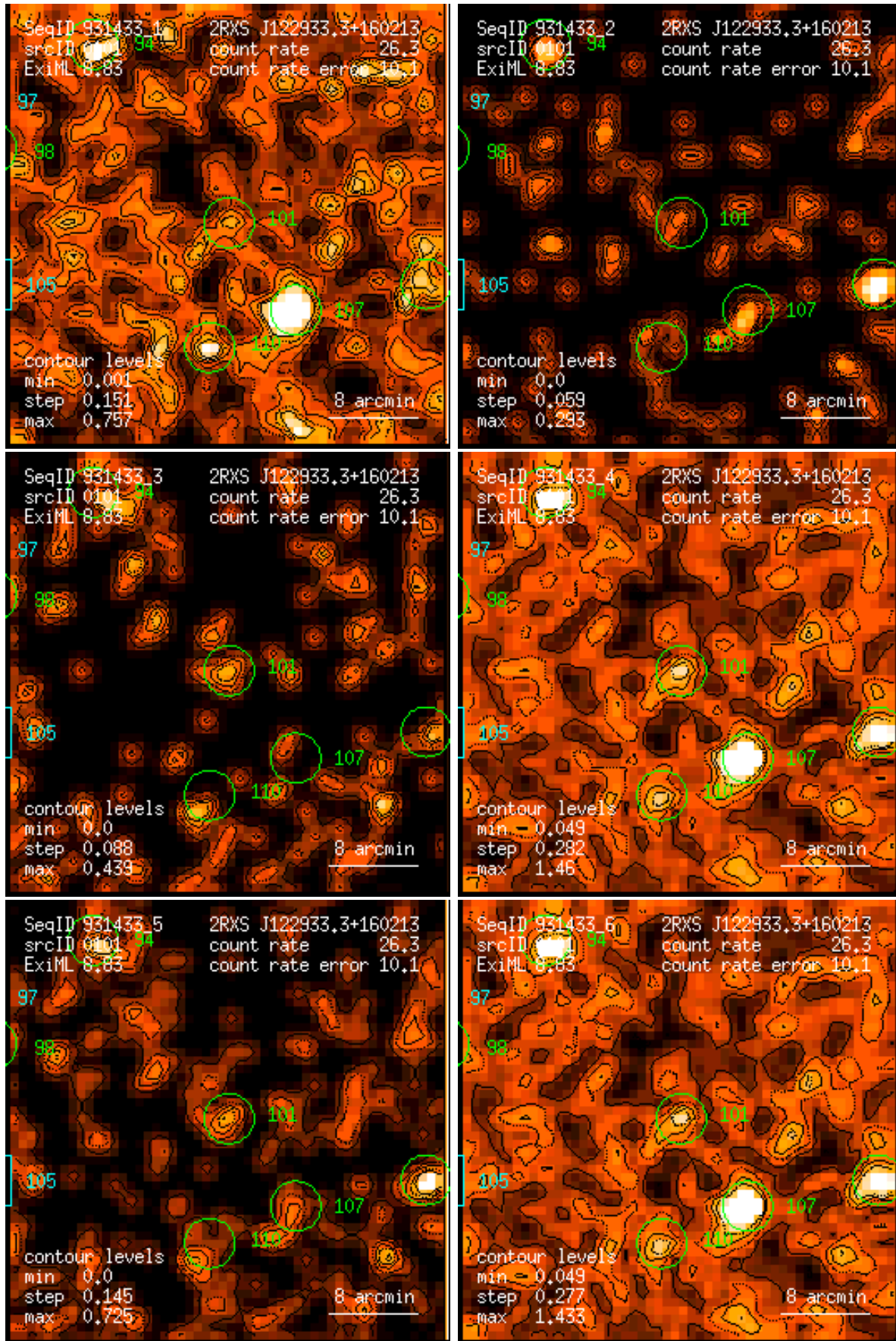
Figure 101: RASS 931433: detection 0101: band rate images, Gaussian filter: (1) PSPC channels 11 – 41, (2) 52 – 90, (3) 91 – 201, (4) 11 – 235, (5) 52 – 201, (6) 11 – 201. Broad band rates in counts/ks. Band rate contour levels in counts/ks/arcmin 2 .
