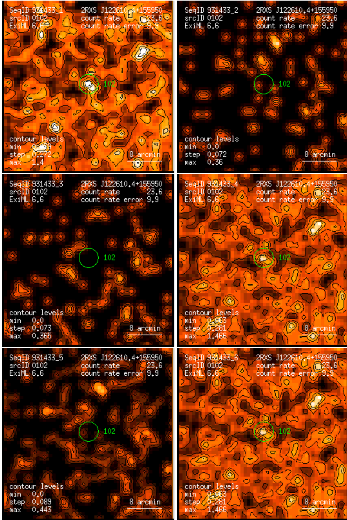
Figure 102: RASS 931433: detection 0102: band rate images, Gaussian filter: (1) PSPC channels 11 – 41, (2) 52 – 90, (3) 91 – 201, (4) 11 – 235, (5) 52 – 201, (6) 11 – 201. Broad band rates in counts/ks. Band rate contour levels in counts/ks/arcmin 2 .
