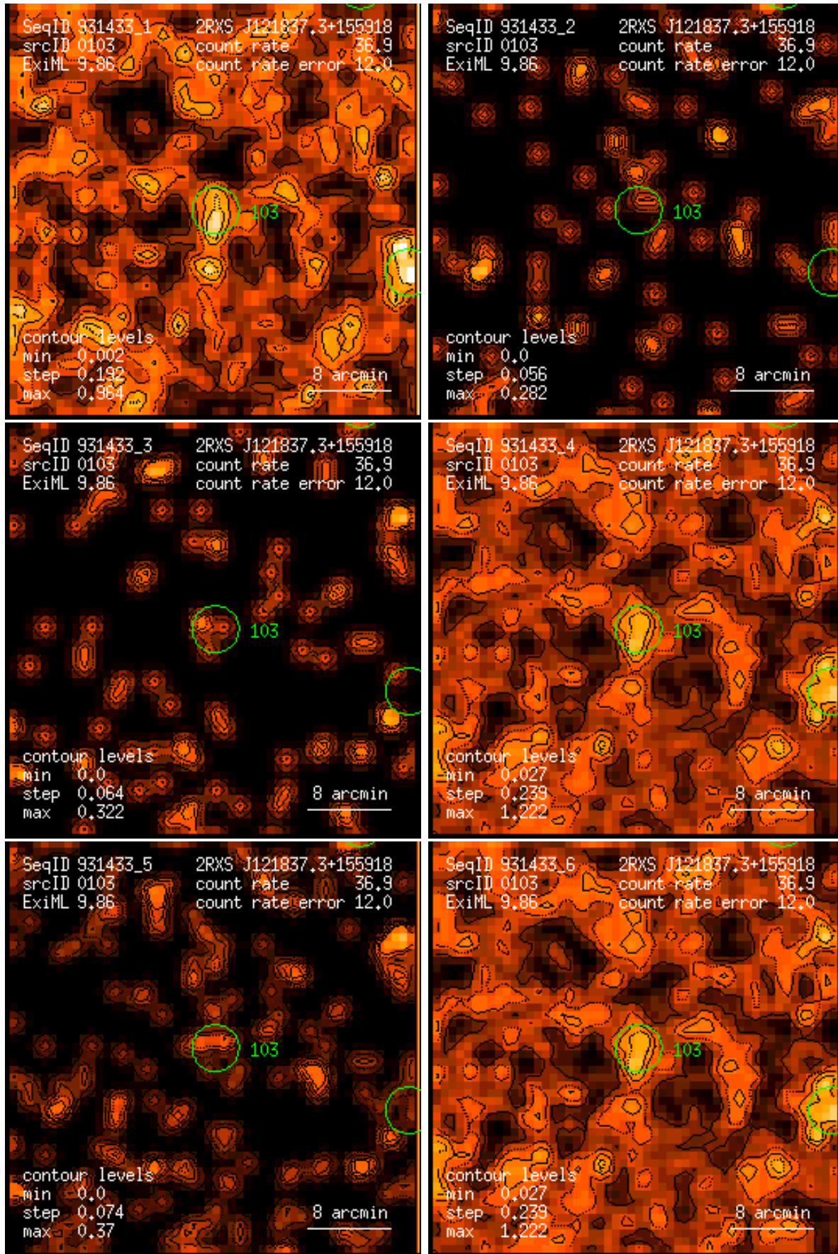
Figure 103: RASS 931433: detection 0103: band rate images, Gaussian filter: (1) PSPC channels 11 – 41, (2) 52 – 90, (3) 91 – 201, (4) 11 – 235, (5) 52 – 201, (6) 11 – 201. Broad band rates in counts/ks. Band rate contour levels in counts/ks/arcmin 2 .
