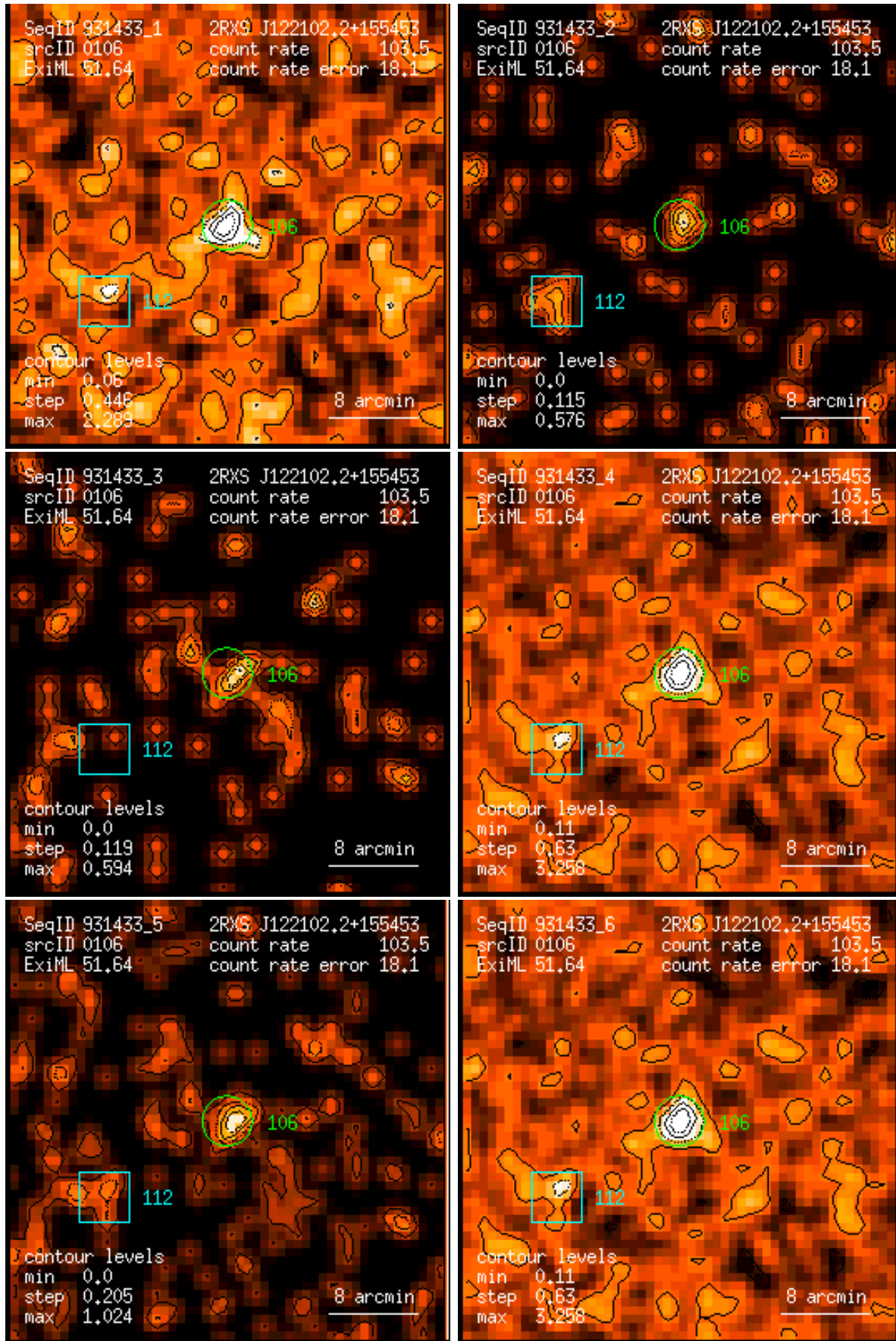
Figure 106: RASS 931433: detection 0106: band rate images, Gaussian filter: (1) PSPC channels 11 – 41, (2) 52 – 90, (3) 91 – 201, (4) 11 – 235, (5) 52 – 201, (6) 11 – 201. Broad band rates in counts/ks. Band rate contour levels in counts/ks/arcmin 2 .
