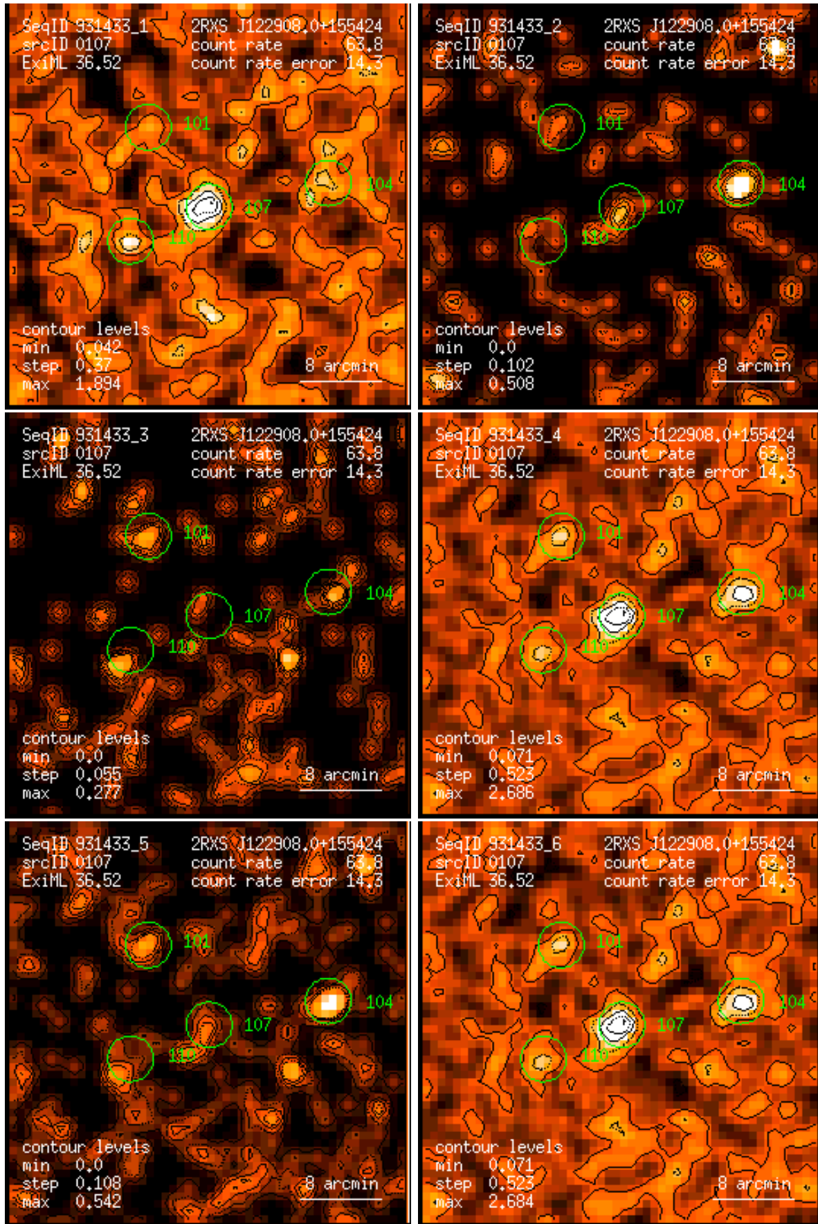
Figure 107: RASS 931433: detection 0107: band rate images, Gaussian filter: (1) PSPC channels 11 – 41, (2) 52 – 90, (3) 91 – 201, (4) 11 – 235, (5) 52 – 201, (6) 11 – 201. Broad band rates in counts/ks. Band rate contour levels in counts/ks/arcmin 2 .
