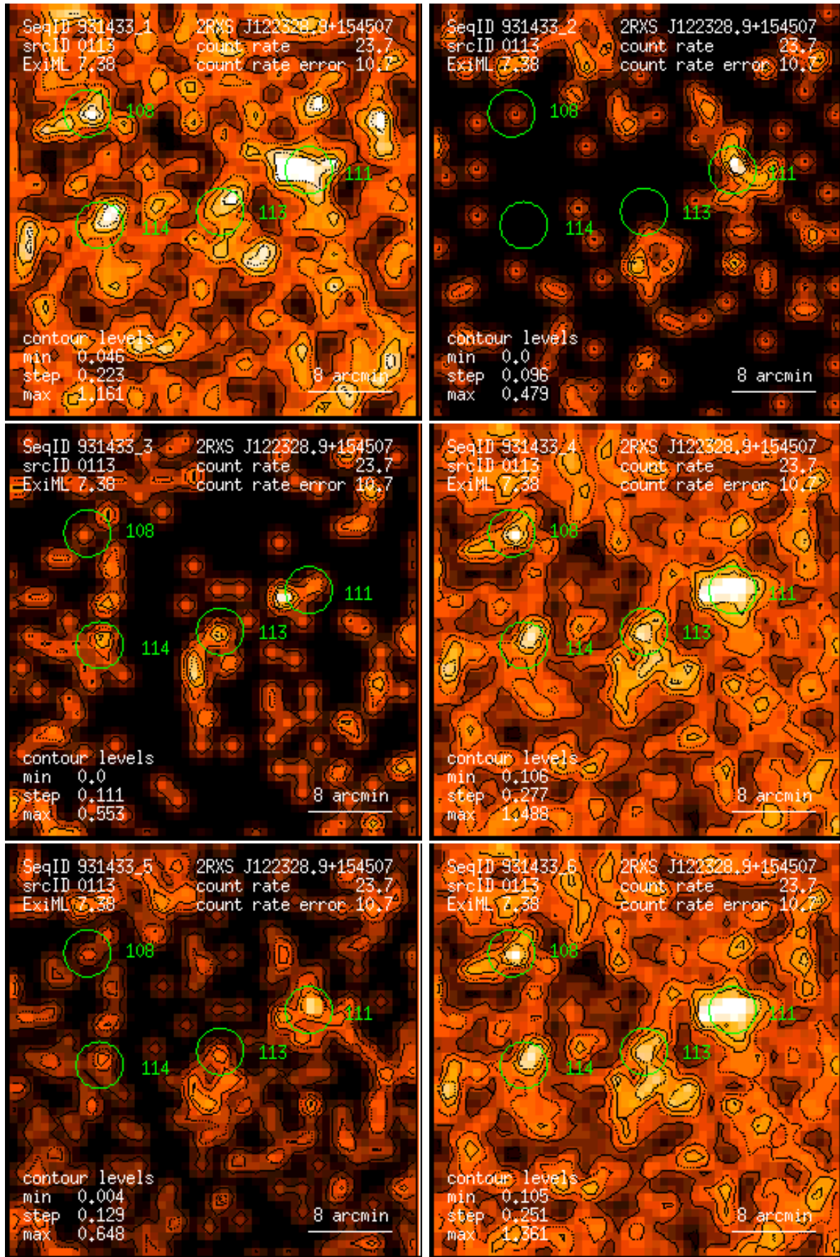
Figure 113: RASS 931433: detection 0113: band rate images, Gaussian filter: (1) PSPC channels 11 – 41, (2) 52 – 90, (3) 91 – 201, (4) 11 – 235, (5) 52 – 201, (6) 11 – 201. Broad band rates in counts/ks. Band rate contour levels in counts/ks/arcmin 2 .
