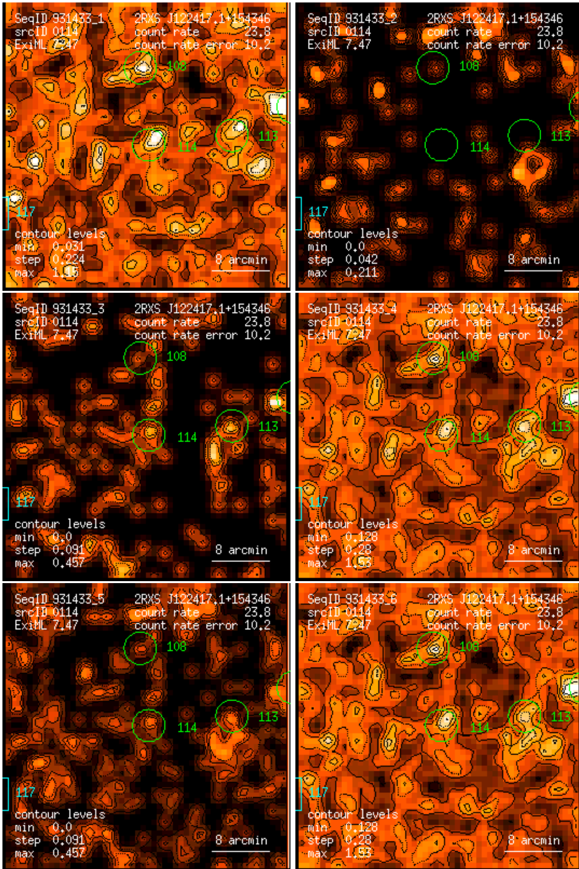
Figure 114: RASS 931433: detection 0114: band rate images, Gaussian filter: (1) PSPC channels 11 – 41, (2) 52 – 90, (3) 91 – 201, (4) 11 – 235, (5) 52 – 201, (6) 11 – 201. Broad band rates in counts/ks. Band rate contour levels in counts/ks/arcmin 2 .
