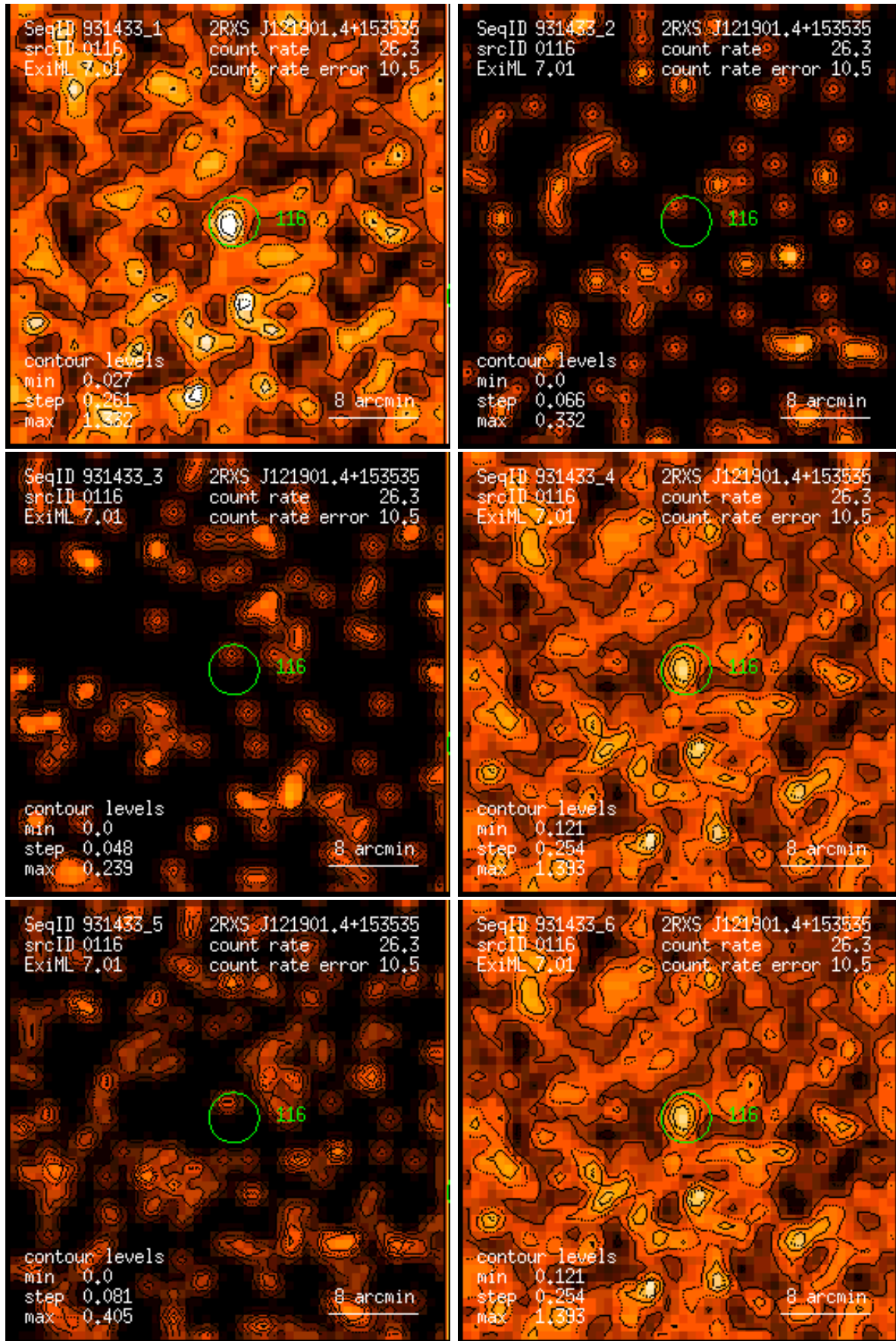
Figure 116: RASS 931433: detection 0116: band rate images, Gaussian filter: (1) PSPC channels 11 – 41, (2) 52 – 90, (3) 91 – 201, (4) 11 – 235, (5) 52 – 201, (6) 11 – 201. Broad band rates in counts/ks. Band rate contour levels in counts/ks/arcmin 2 .
