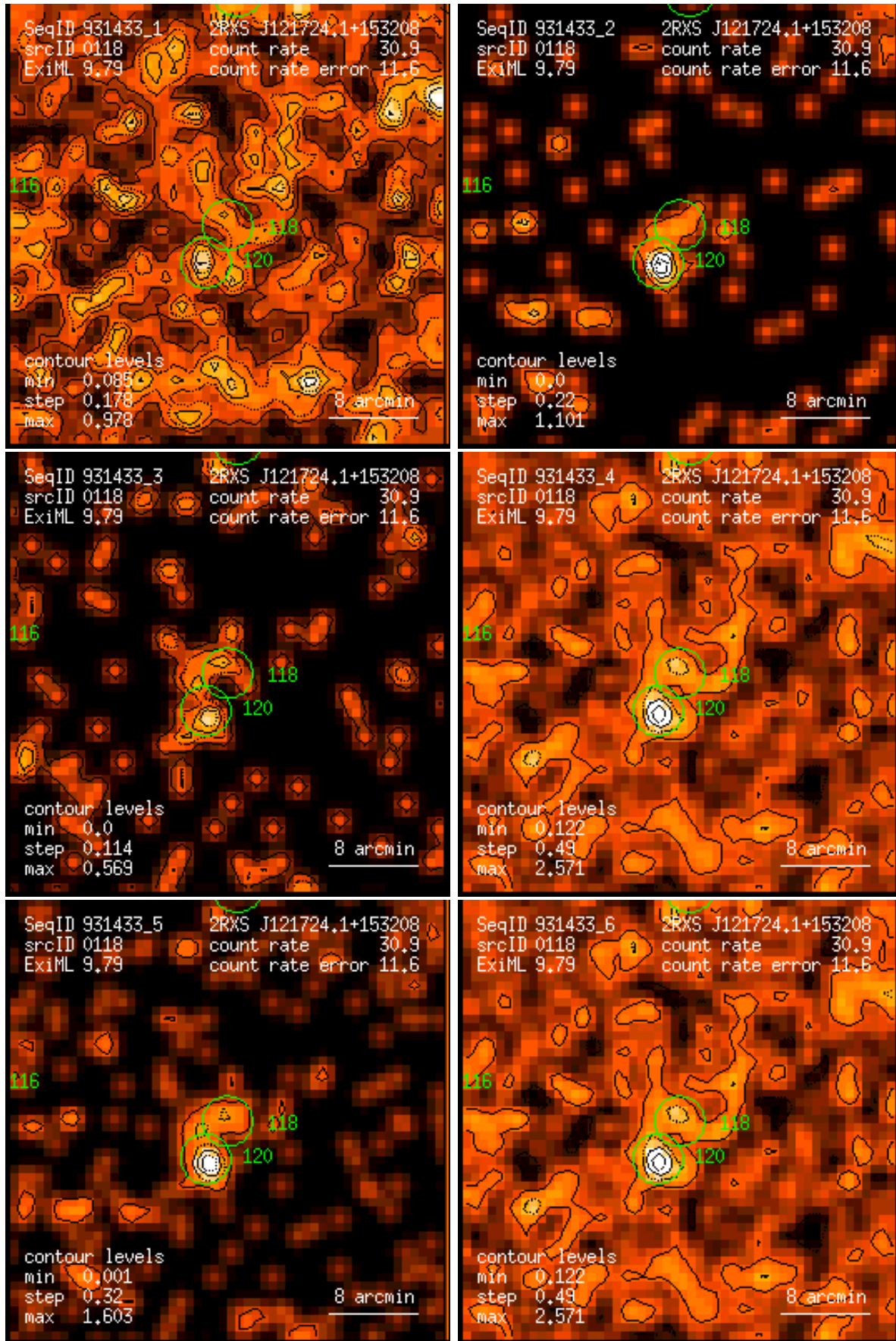
Figure 118: RASS 931433: detection 0118: band rate images, Gaussian filter: (1) PSPC channels 11 – 41, (2) 52 – 90, (3) 91 – 201, (4) 11 – 235, (5) 52 – 201, (6) 11 – 201. Broad band rates in counts/ks. Band rate contour levels in counts/ks/arcmin 2 .
