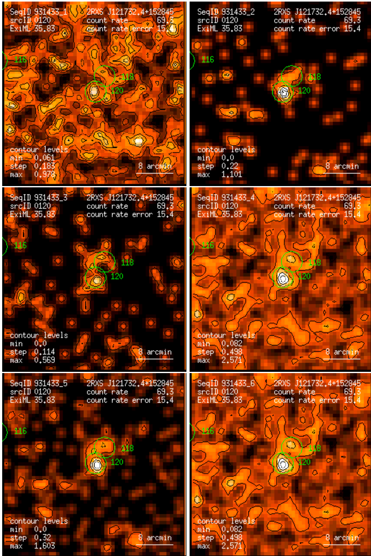
Figure 120: RASS 931433: detection 0120: band rate images, Gaussian filter: (1) PSPC channels 11 – 41, (2) 52 – 90, (3) 91 – 201, (4) 11 – 235, (5) 52 – 201, (6) 11 – 201. Broad band rates in counts/ks. Band rate contour levels in counts/ks/arcmin 2 .
