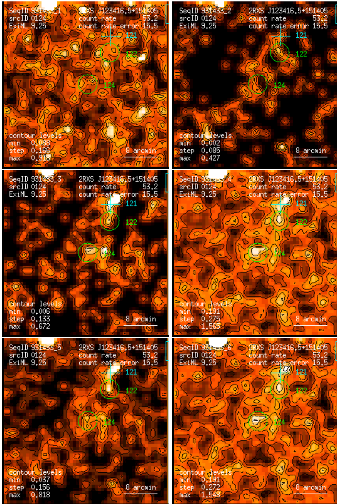
Figure 124: RASS 931433: detection 0124: band rate images, Gaussian filter: (1) PSPC channels 11 – 41, (2) 52 – 90, (3) 91 – 201, (4) 11 – 235, (5) 52 – 201, (6) 11 – 201. Broad band rates in counts/ks. Band rate contour levels in counts/ks/arcmin 2 .
