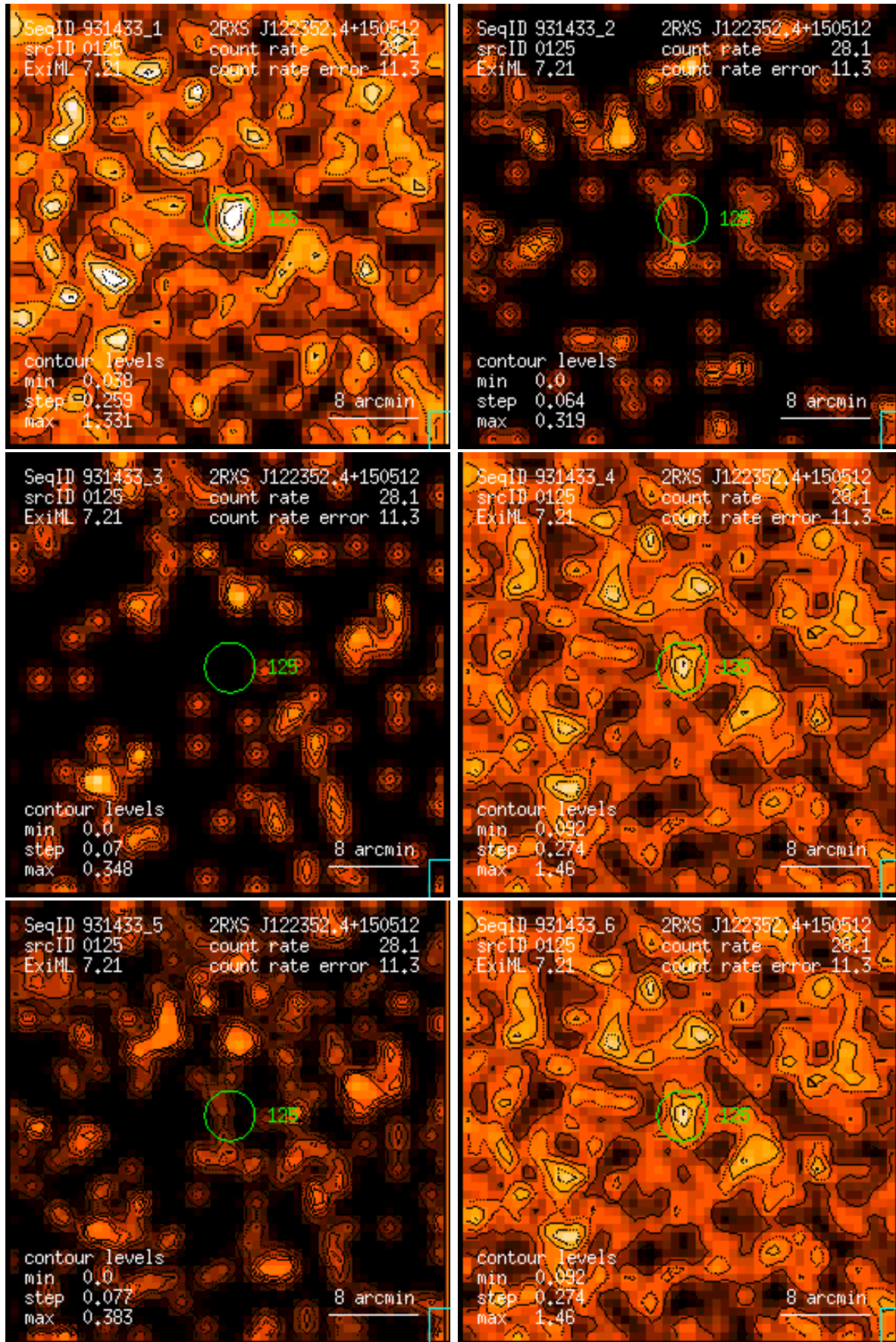
Figure 125: RASS 931433: detection 0125: band rate images, Gaussian filter: (1) PSPC channels 11 – 41, (2) 52 – 90, (3) 91 – 201, (4) 11 – 235, (5) 52 – 201, (6) 11 – 201. Broad band rates in counts/ks. Band rate contour levels in counts/ks/arcmin 2 .
