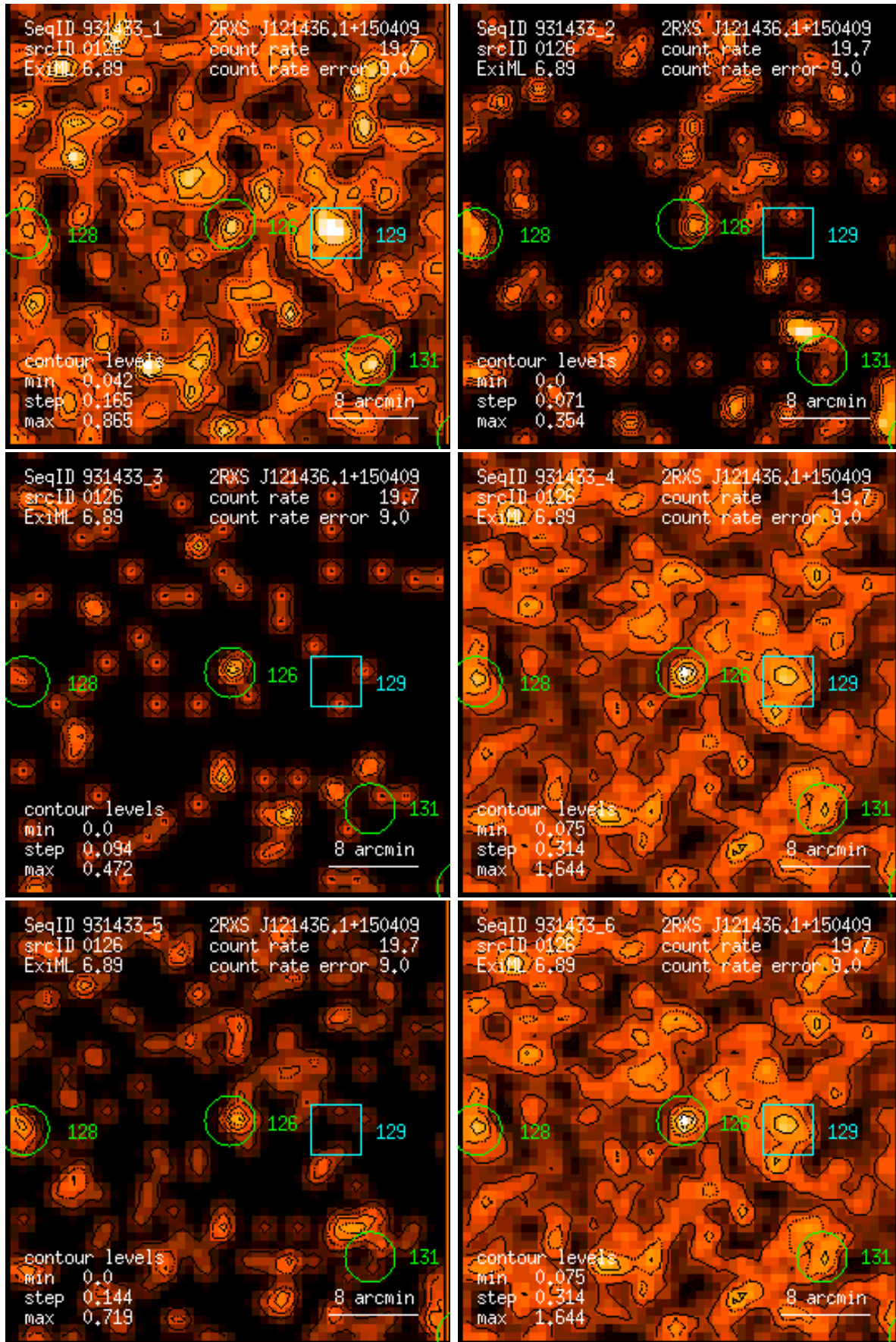
Figure 126: RASS 931433: detection 0126: band rate images, Gaussian filter: (1) PSPC channels 11 – 41, (2) 52 – 90, (3) 91 – 201, (4) 11 – 235, (5) 52 – 201, (6) 11 – 201. Broad band rates in counts/ks. Band rate contour levels in counts/ks/arcmin 2 .
