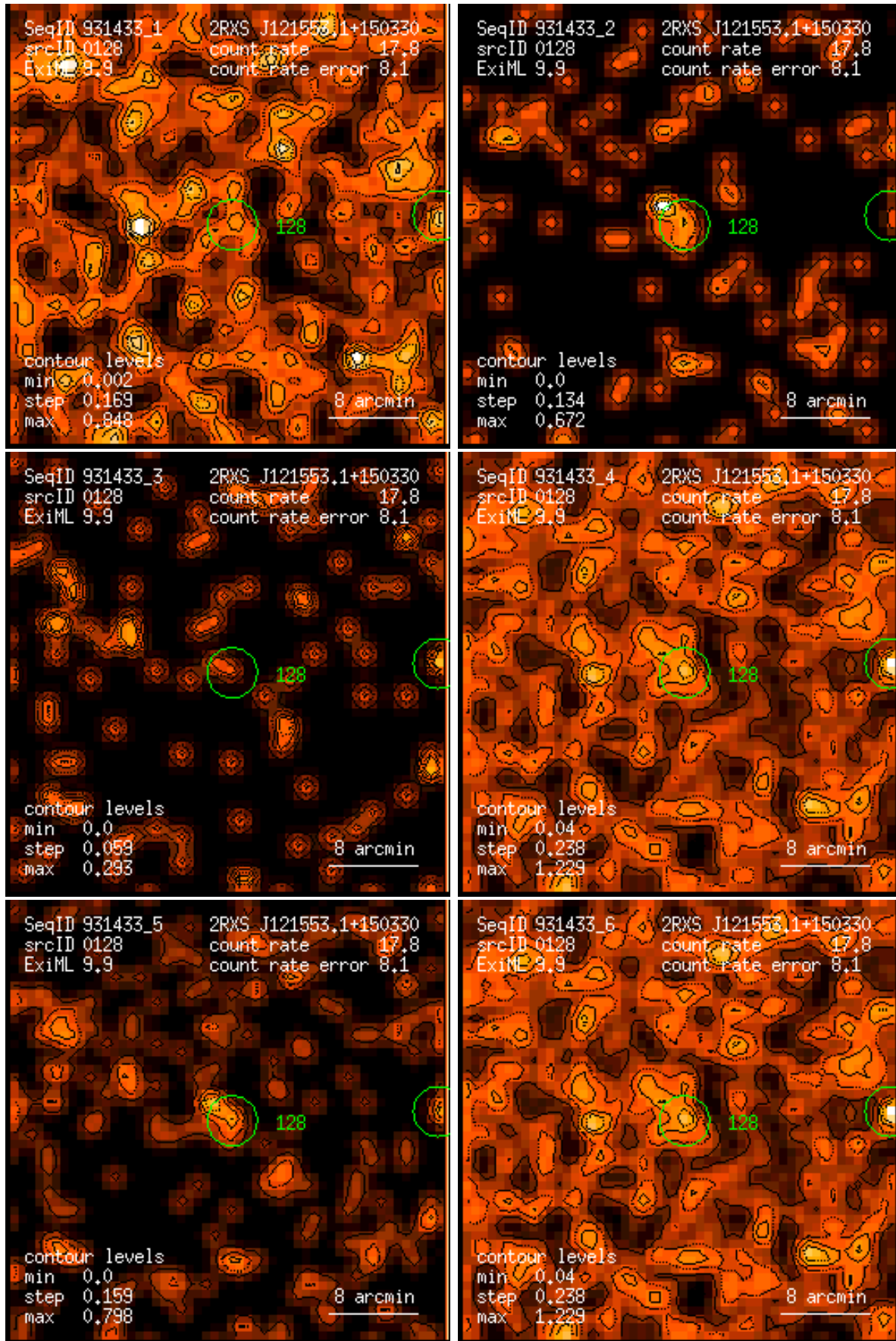
Figure 128: RASS 931433: detection 0128: band rate images, Gaussian filter: (1) PSPC channels 11 – 41, (2) 52 – 90, (3) 91 – 201, (4) 11 – 235, (5) 52 – 201, (6) 11 – 201. Broad band rates in counts/ks. Band rate contour levels in counts/ks/arcmin 2 .
