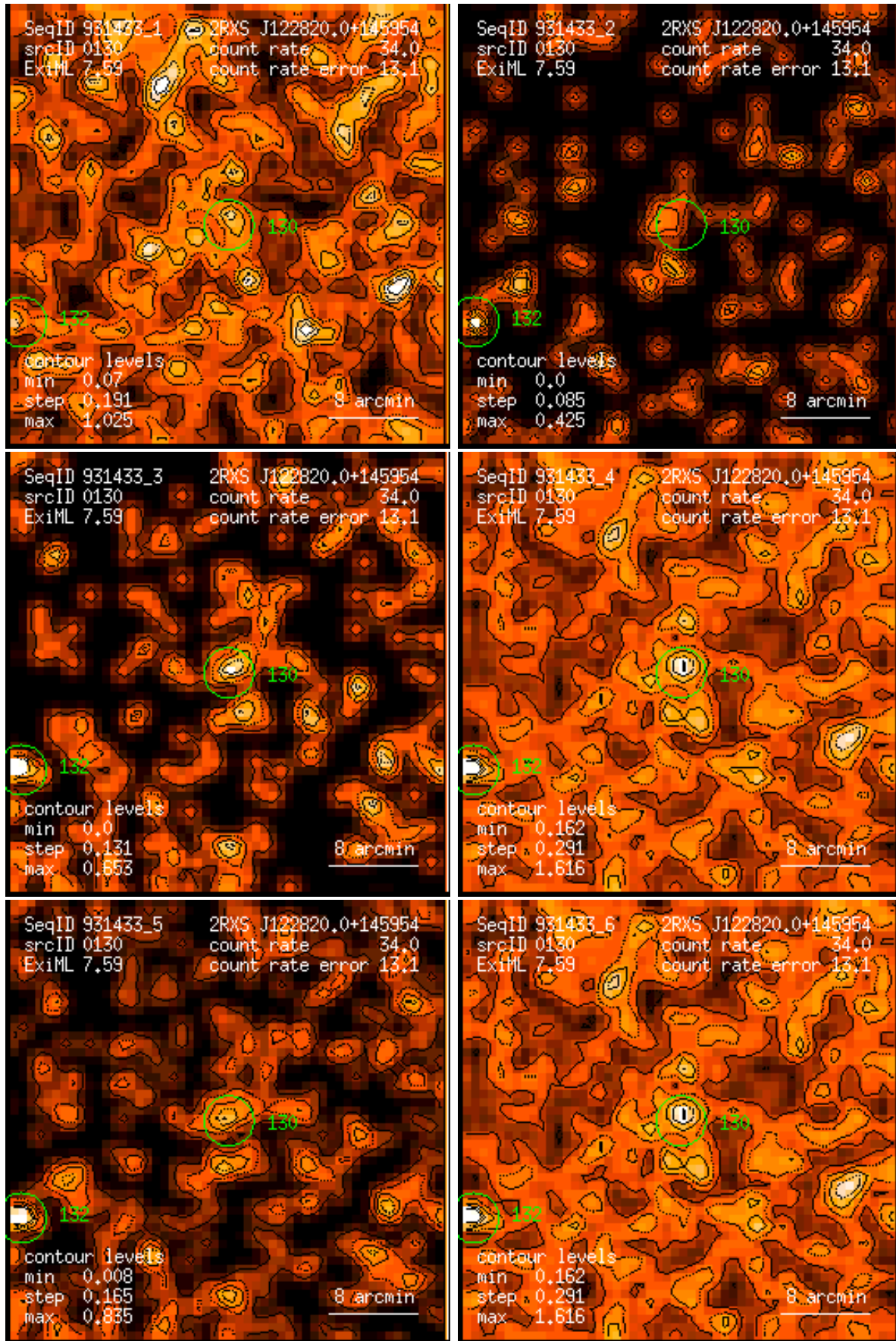
Figure 130: RASS 931433: detection 0130: band rate images, Gaussian filter: (1) PSPC channels 11 – 41, (2) 52 – 90, (3) 91 – 201, (4) 11 – 235, (5) 52 – 201, (6) 11 – 201. Broad band rates in counts/ks. Band rate contour levels in counts/ks/arcmin 2 .
