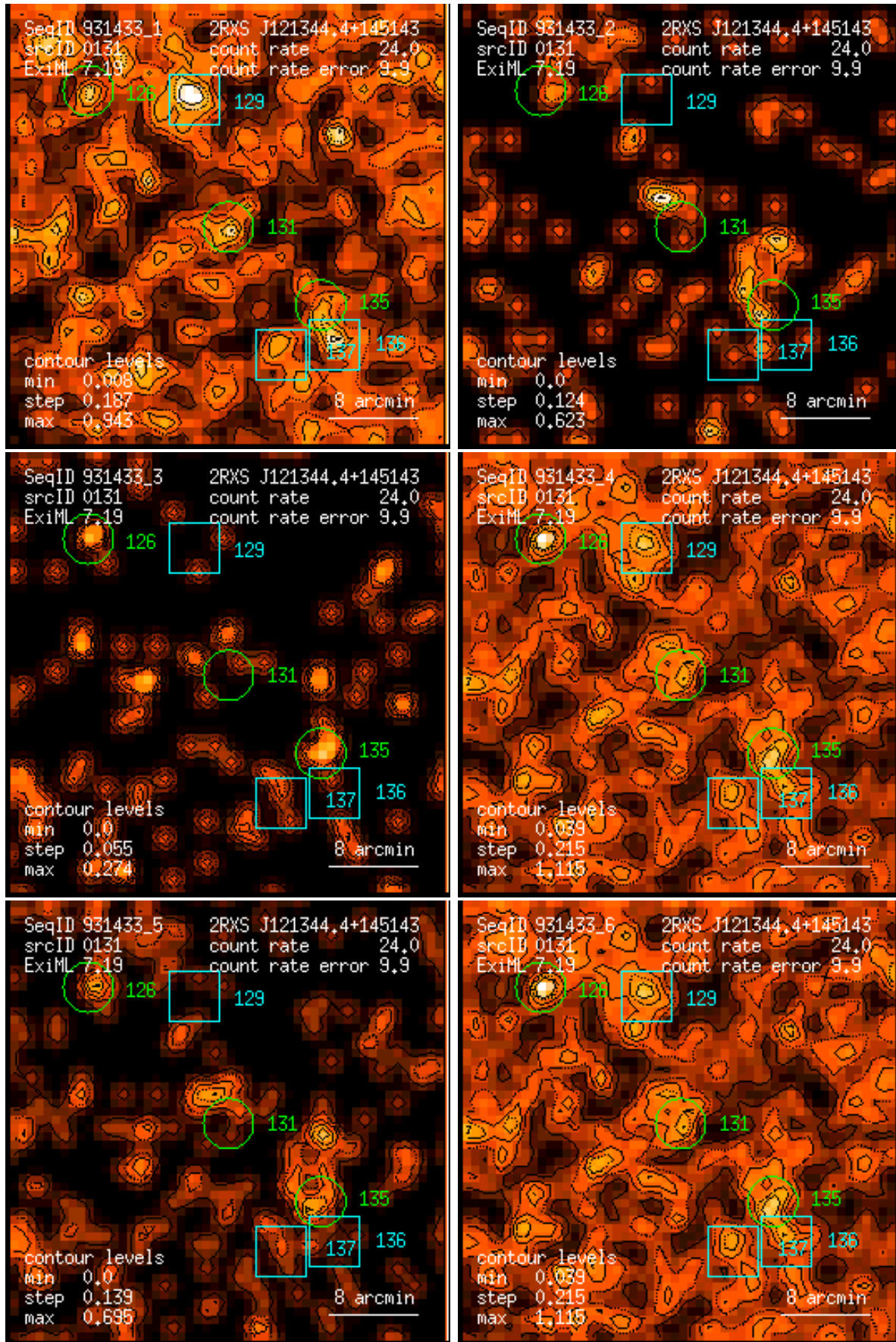
Figure 131: RASS 931433: detection 0131: band rate images, Gaussian filter: (1) PSPC channels 11 – 41, (2) 52 – 90, (3) 91 – 201, (4) 11 – 235, (5) 52 – 201, (6) 11 – 201. Broad band rates in counts/ks. Band rate contour levels in counts/ks/arcmin 2 .
