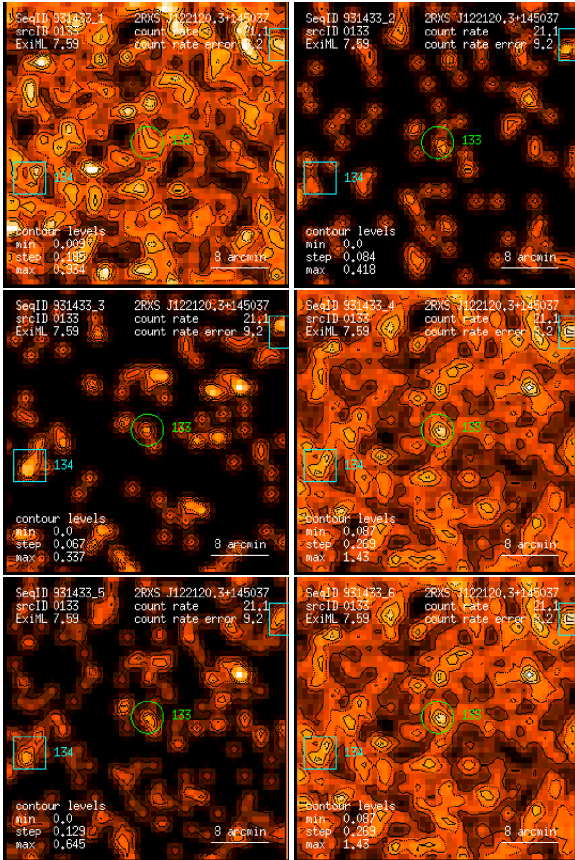
Figure 133: RASS 931433: detection 0133: band rate images, Gaussian filter: (1) PSPC channels 11 – 41, (2) 52 – 90, (3) 91 – 201, (4) 11 – 235, (5) 52 – 201, (6) 11 – 201. Broad band rates in counts/ks. Band rate contour levels in counts/ks/arcmin 2 .
