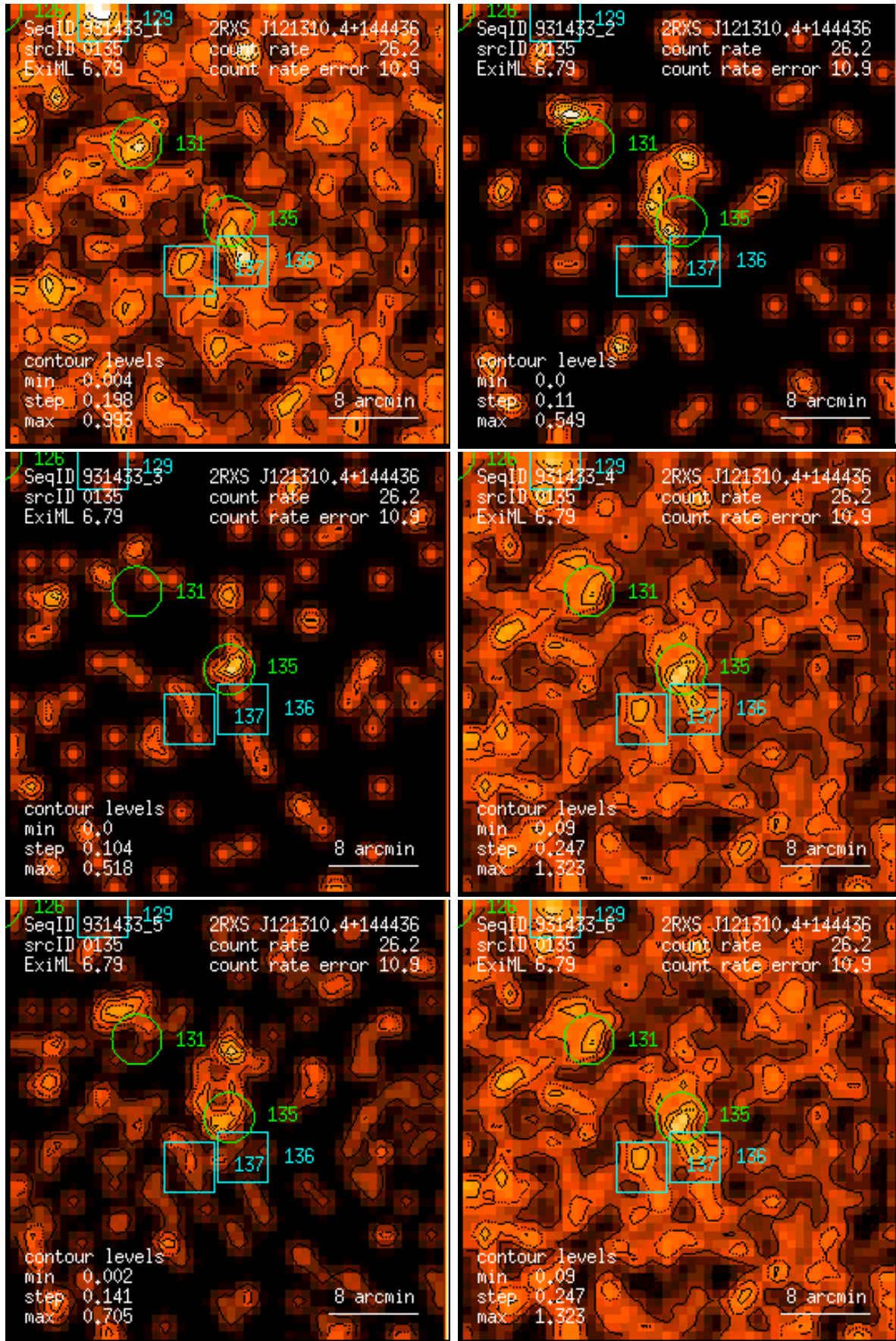
Figure 135: RASS 931433: detection 0135: band rate images, Gaussian filter: (1) PSPC channels 11 – 41, (2) 52 – 90, (3) 91 – 201, (4) 11 – 235, (5) 52 – 201, (6) 11 – 201. Broad band rates in counts/ks. Band rate contour levels in counts/ks/arcmin 2 .
