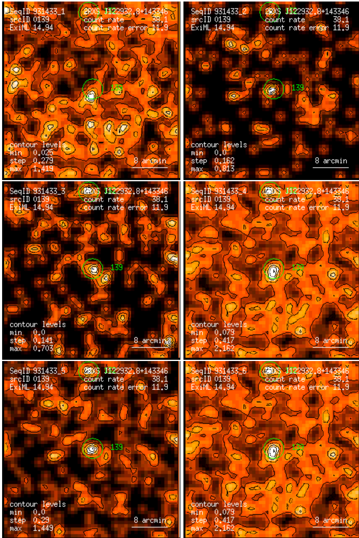
Figure 139: RASS 931433: detection 0139: band rate images, Gaussian filter: (1) PSPC channels 11 – 41, (2) 52 – 90, (3) 91 – 201, (4) 11 – 235, (5) 52 – 201, (6) 11 – 201. Broad band rates in counts/ks. Band rate contour levels in counts/ks/arcmin 2 .
