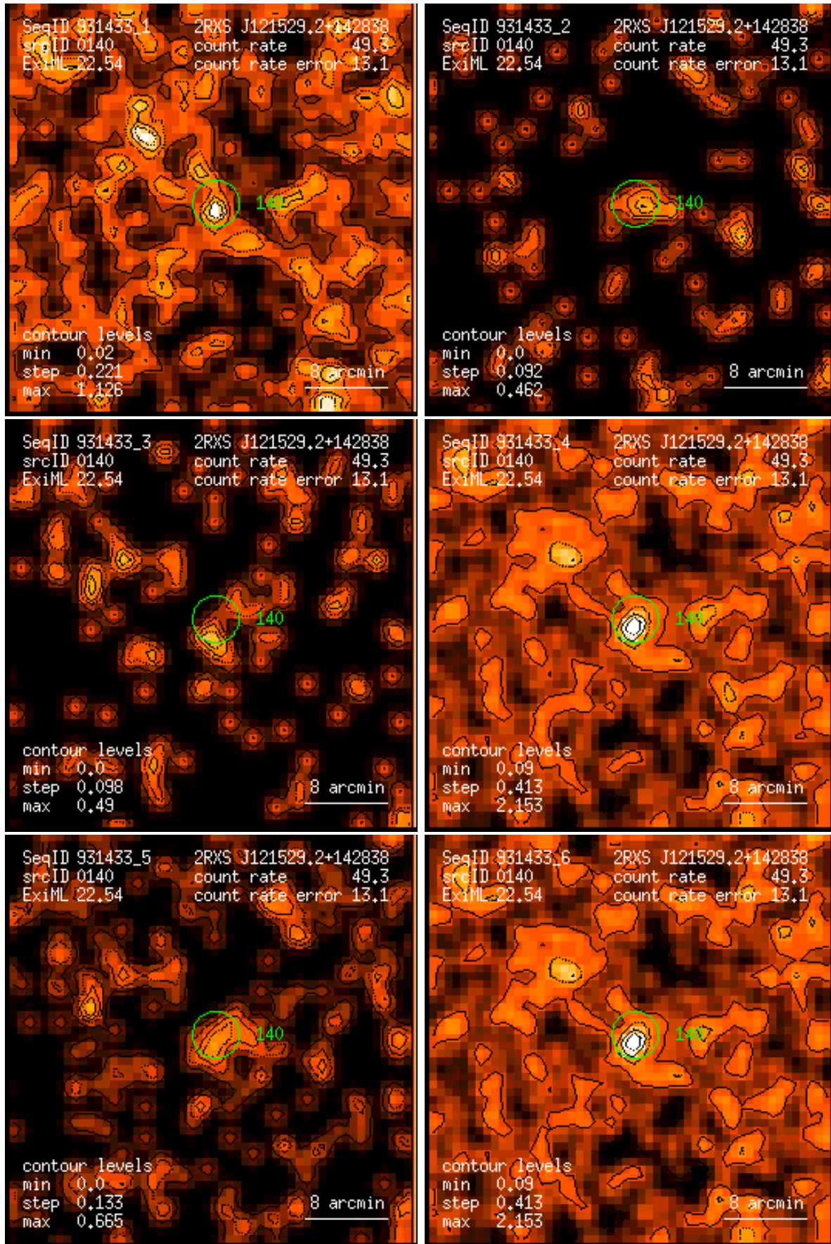
Figure 140: RASS 931433: detection 0140: band rate images, Gaussian filter: (1) PSPC channels 11 – 41, (2) 52 – 90, (3) 91 – 201, (4) 11 – 235, (5) 52 – 201, (6) 11 – 201. Broad band rates in counts/ks. Band rate contour levels in counts/ks/arcmin 2 .
