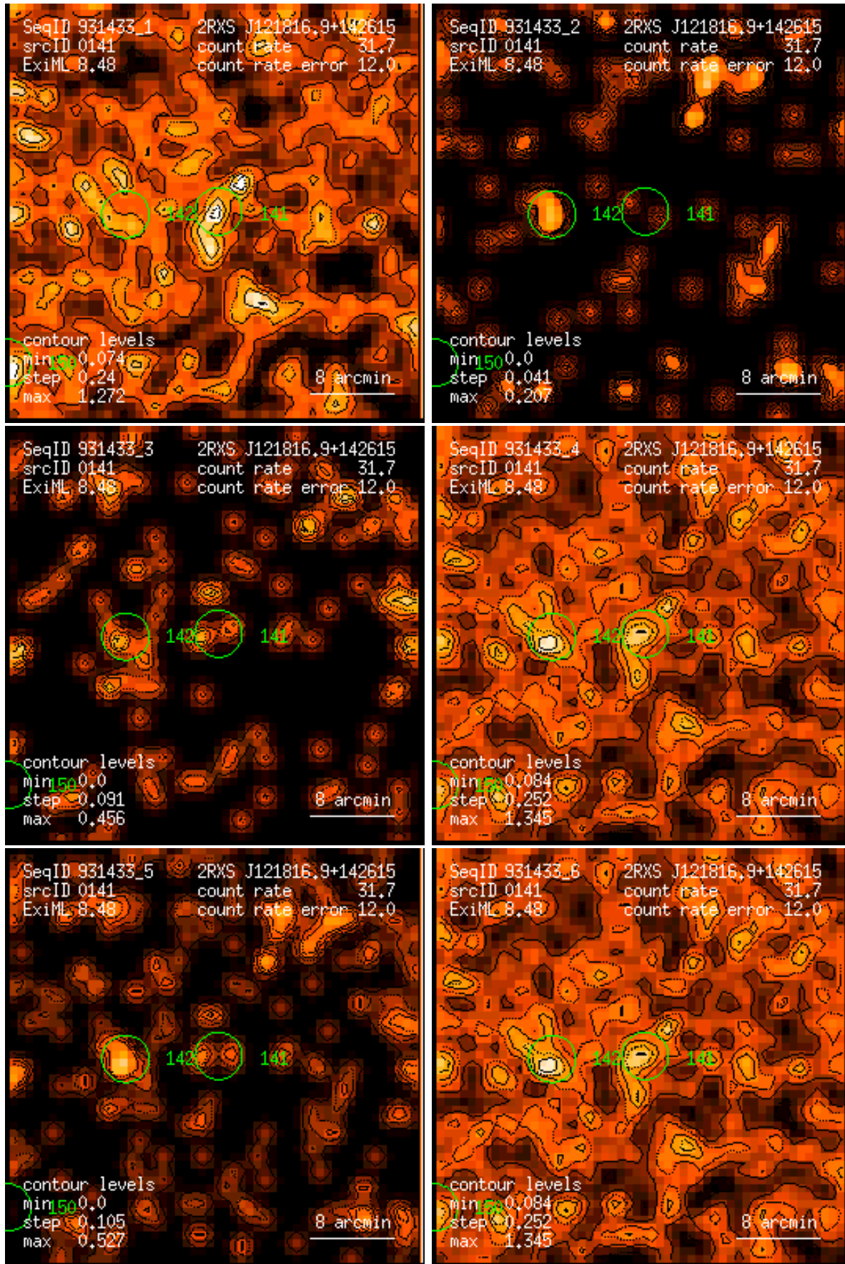
Figure 141: RASS 931433: detection 0141: band rate images, Gaussian filter: (1) PSPC channels 11 – 41, (2) 52 – 90, (3) 91 – 201, (4) 11 – 235, (5) 52 – 201, (6) 11 – 201. Broad band rates in counts/ks. Band rate contour levels in counts/ks/arcmin 2 .
