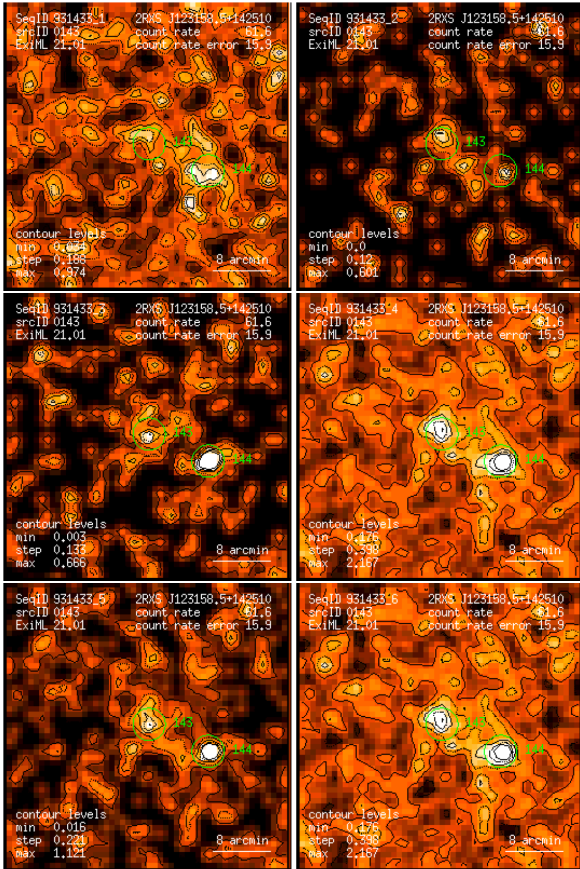
Figure 143: RASS 931433: detection 0143: band rate images, Gaussian filter: (1) PSPC channels 11 – 41, (2) 52 – 90, (3) 91 – 201, (4) 11 – 235, (5) 52 – 201, (6) 11 – 201. Broad band rates in counts/ks. Band rate contour levels in counts/ks/arcmin 2 .
