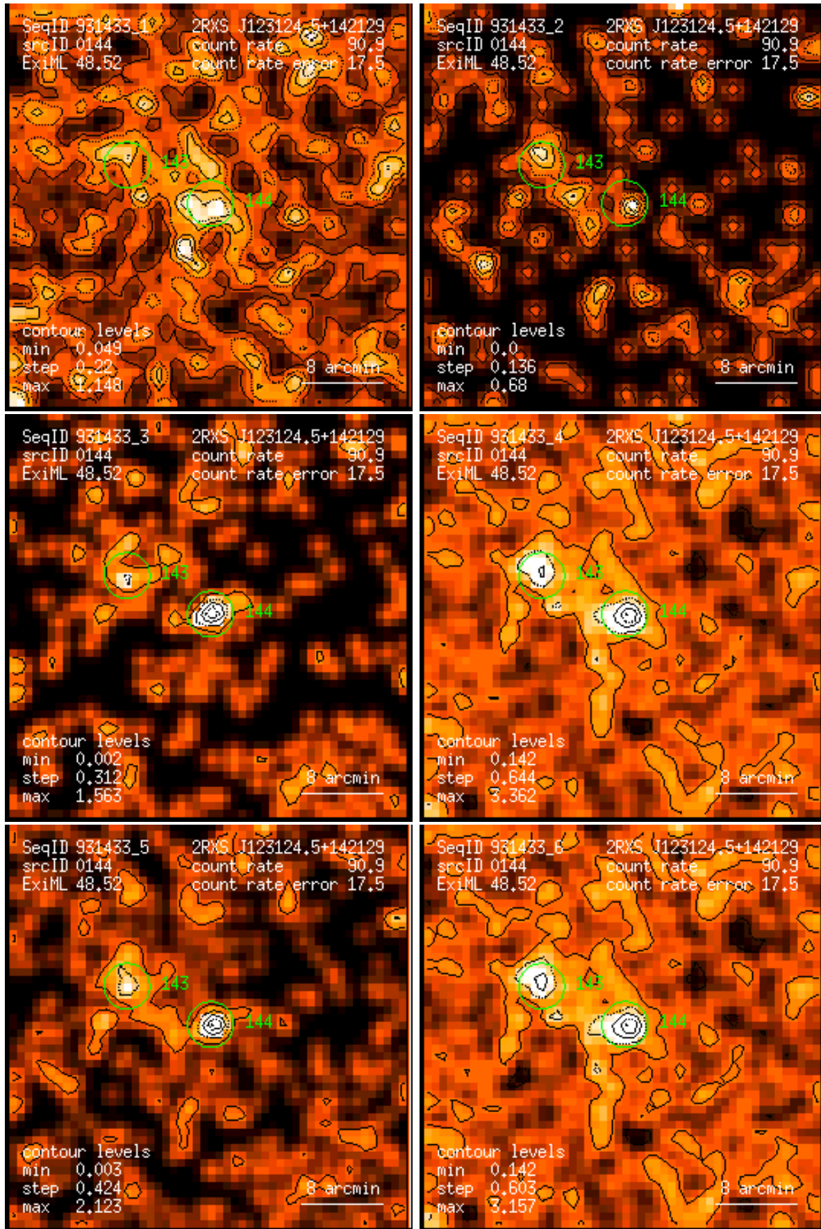
Figure 144: RASS 931433: detection 0144: band rate images, Gaussian filter: (1) PSPC channels 11 – 41, (2) 52 – 90, (3) 91 – 201, (4) 11 – 235, (5) 52 – 201, (6) 11 – 201. Broad band rates in counts/ks. Band rate contour levels in counts/ks/arcmin 2 .
