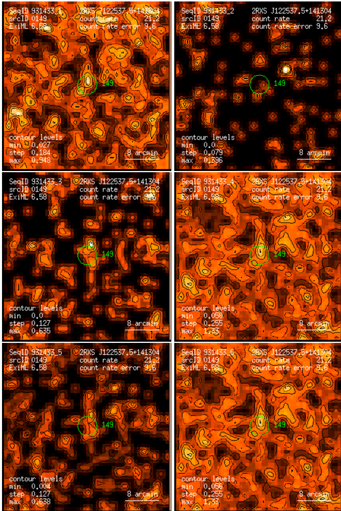
Figure 149: RASS 931433: detection 0149: band rate images, Gaussian filter: (1) PSPC channels 11 – 41, (2) 52 – 90, (3) 91 – 201, (4) 11 – 235, (5) 52 – 201, (6) 11 – 201. Broad band rates in counts/ks. Band rate contour levels in counts/ks/arcmin 2 .
