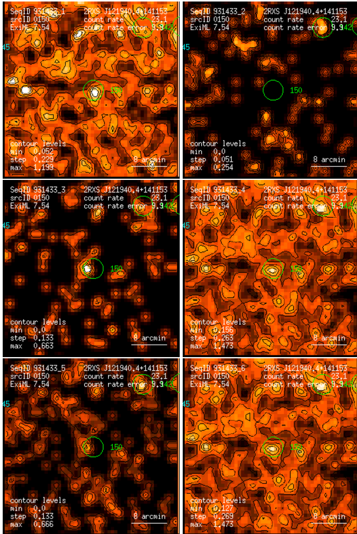
Figure 150: RASS 931433: detection 0150: band rate images, Gaussian filter: (1) PSPC channels 11 – 41, (2) 52 – 90, (3) 91 – 201, (4) 11 – 235, (5) 52 – 201, (6) 11 – 201. Broad band rates in counts/ks. Band rate contour levels in counts/ks/arcmin 2 .
