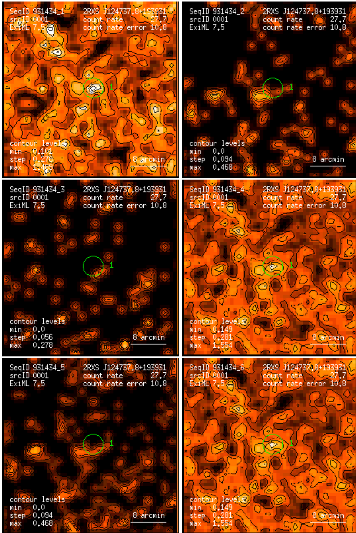
Figure 1: RASS 931434: detection 0001: band rate images, Gaussian filter: (1) PSPC channels 11 – 41, (2) 52 – 90, (3) 91 – 201, (4) 11 – 235, (5) 52 – 201, (6) 11 – 201. Broad band rates in counts/ks. Band rate contour levels in counts/ks/arcmin 2 .
