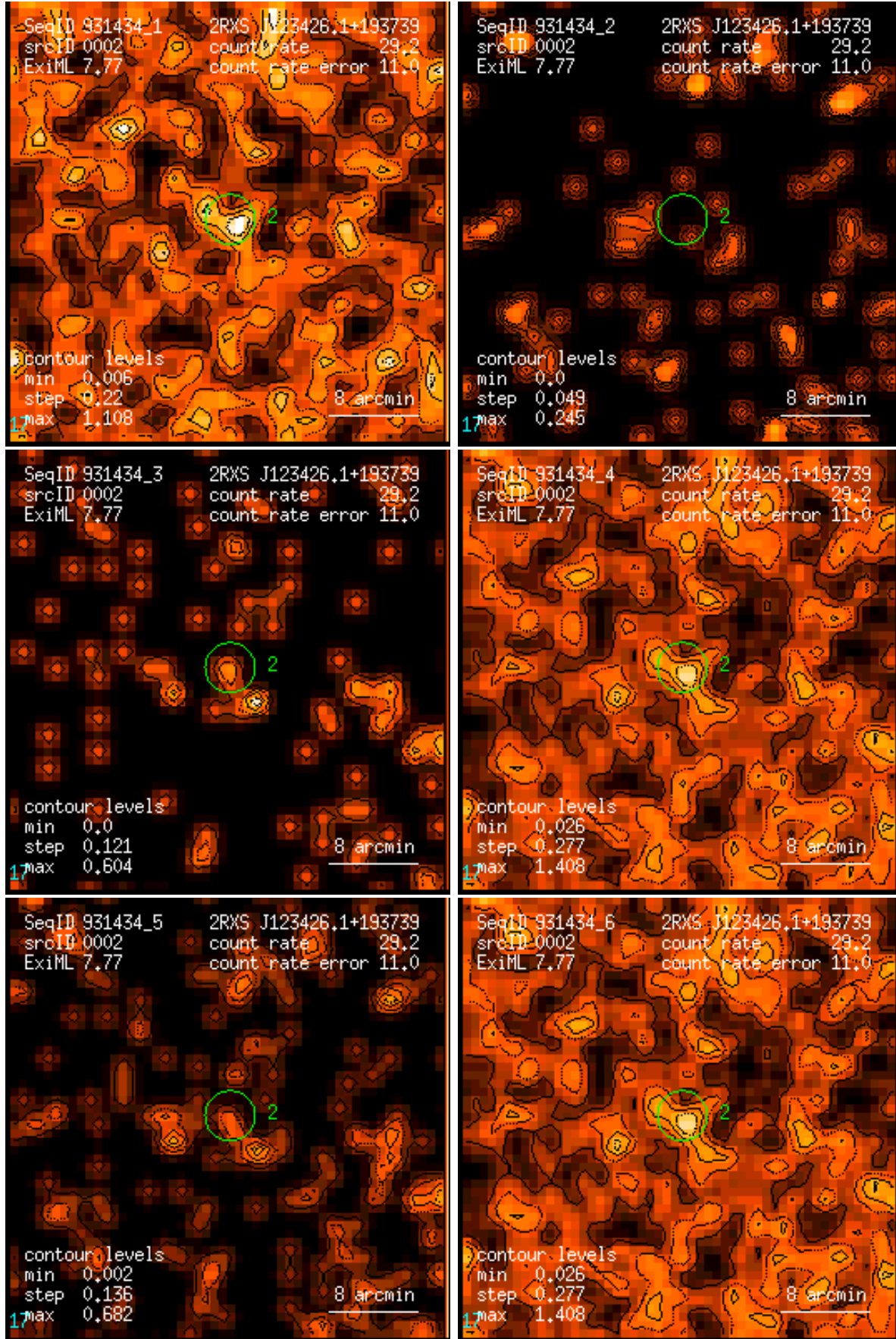
Figure 2: RASS 931434: detection 0002: band rate images, Gaussian filter: (1) PSPC channels 11 – 41, (2) 52 – 90, (3) 91 – 201, (4) 11 – 235, (5) 52 – 201, (6) 11 – 201. Broad band rates in counts/ks. Band rate contour levels in counts/ks/arcmin 2 .
