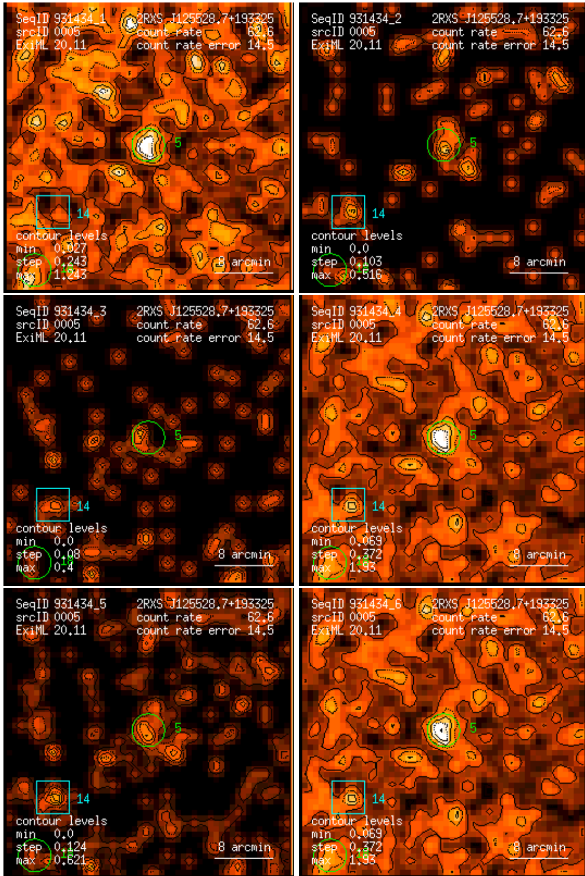
Figure 5: RASS 931434: detection 0005: band rate images, Gaussian filter: (1) PSPC channels 11 – 41, (2) 52 – 90, (3) 91 – 201, (4) 11 – 235, (5) 52 – 201, (6) 11 – 201. Broad band rates in counts/ks. Band rate contour levels in counts/ks/arcmin 2 .
