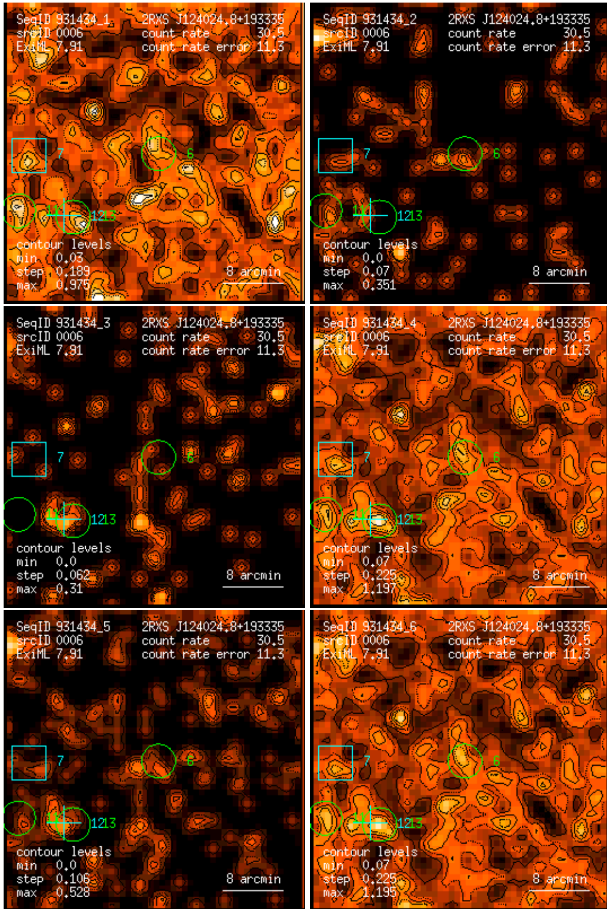
Figure 6: RASS 931434: detection 0006: band rate images, Gaussian filter: (1) PSPC channels 11 – 41, (2) 52 – 90, (3) 91 – 201, (4) 11 – 235, (5) 52 – 201, (6) 11 – 201. Broad band rates in counts/ks. Band rate contour levels in counts/ks/arcmin 2 .
