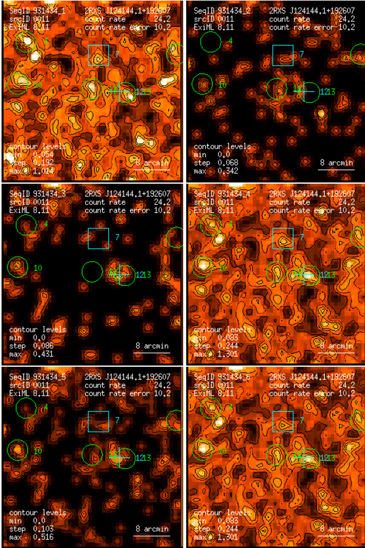
Figure 11: RASS 931434: detection 0011: band rate images, Gaussian filter: (1) PSPC channels 11 – 41, (2) 52 – 90, (3) 91 – 201, (4) 11 – 235, (5) 52 – 201, (6) 11 – 201. Broad band rates in counts/ks. Band rate contour levels in counts/ks/arcmin 2 .
