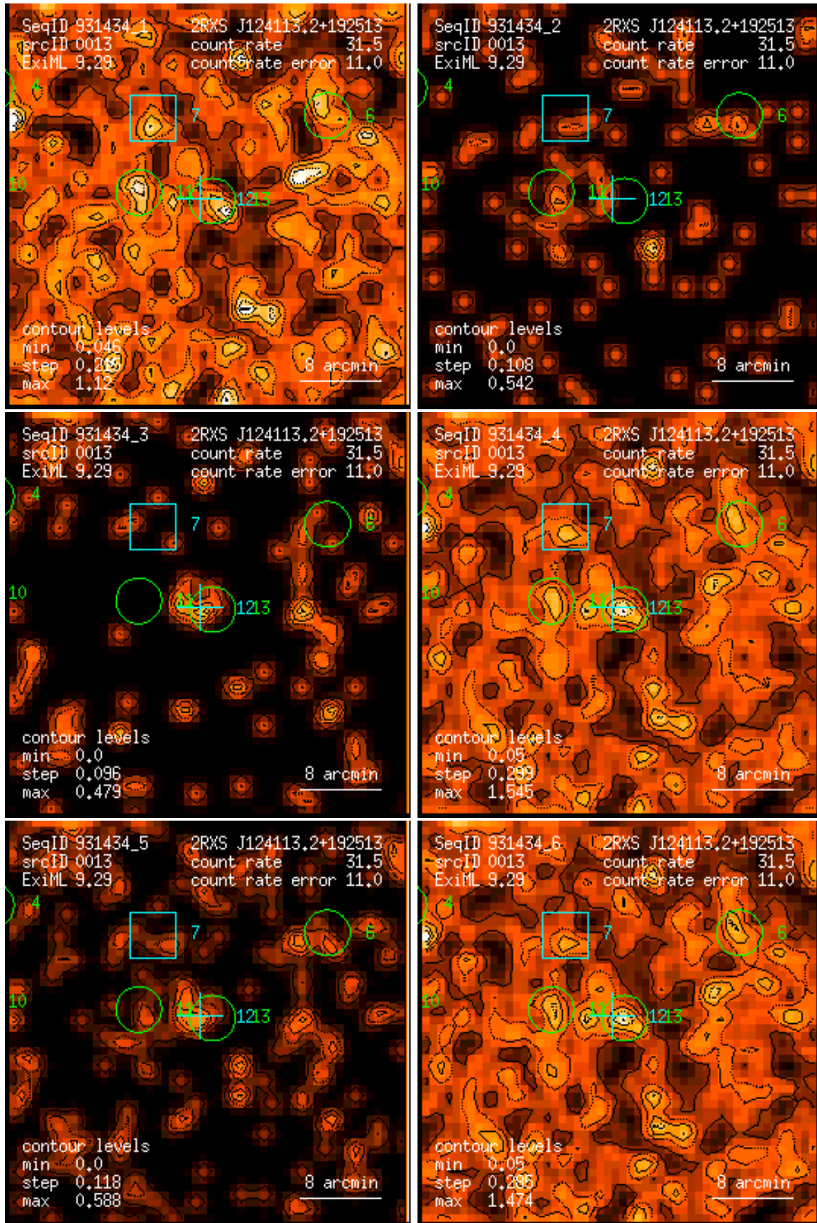
Figure 13: RASS 931434: detection 0013: band rate images, Gaussian filter: (1) PSPC channels 11 – 41, (2) 52 – 90, (3) 91 – 201, (4) 11 – 235, (5) 52 – 201, (6) 11 – 201. Broad band rates in counts/ks. Band rate contour levels in counts/ks/arcmin 2 .
