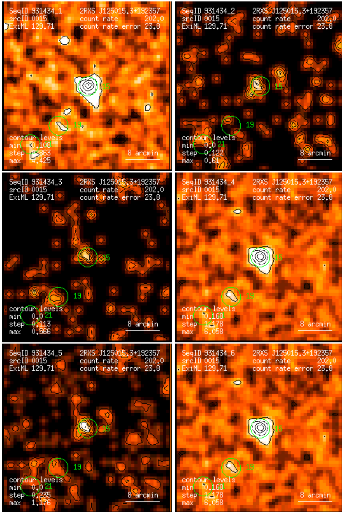
Figure 15: RASS 931434: detection 0015: band rate images, Gaussian filter: (1) PSPC channels 11 – 41, (2) 52 – 90, (3) 91 – 201, (4) 11 – 235, (5) 52 – 201, (6) 11 – 201. Broad band rates in counts/ks. Band rate contour levels in counts/ks/arcmin 2 .
