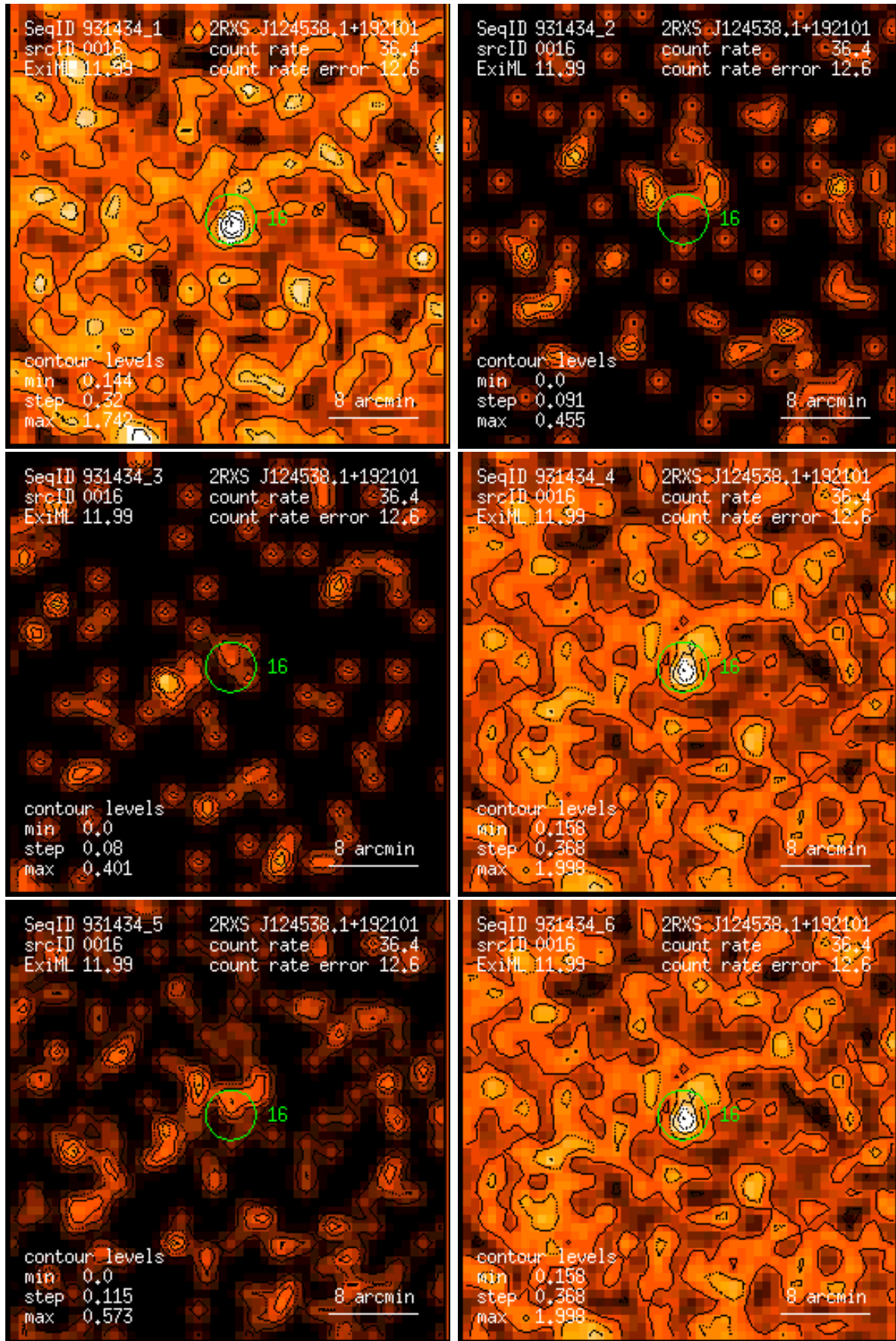
Figure 16: RASS 931434: detection 0016: band rate images, Gaussian filter: (1) PSPC channels 11 – 41, (2) 52 – 90, (3) 91 – 201, (4) 11 – 235, (5) 52 – 201, (6) 11 – 201. Broad band rates in counts/ks. Band rate contour levels in counts/ks/arcmin 2 .
