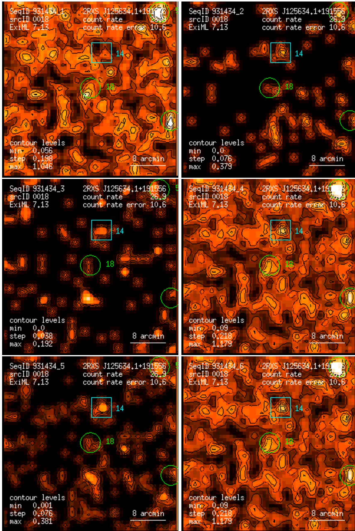
Figure 18: RASS 931434: detection 0018: band rate images, Gaussian filter: (1) PSPC channels 11 – 41, (2) 52 – 90, (3) 91 – 201, (4) 11 – 235, (5) 52 – 201, (6) 11 – 201. Broad band rates in counts/ks. Band rate contour levels in counts/ks/arcmin 2 .
