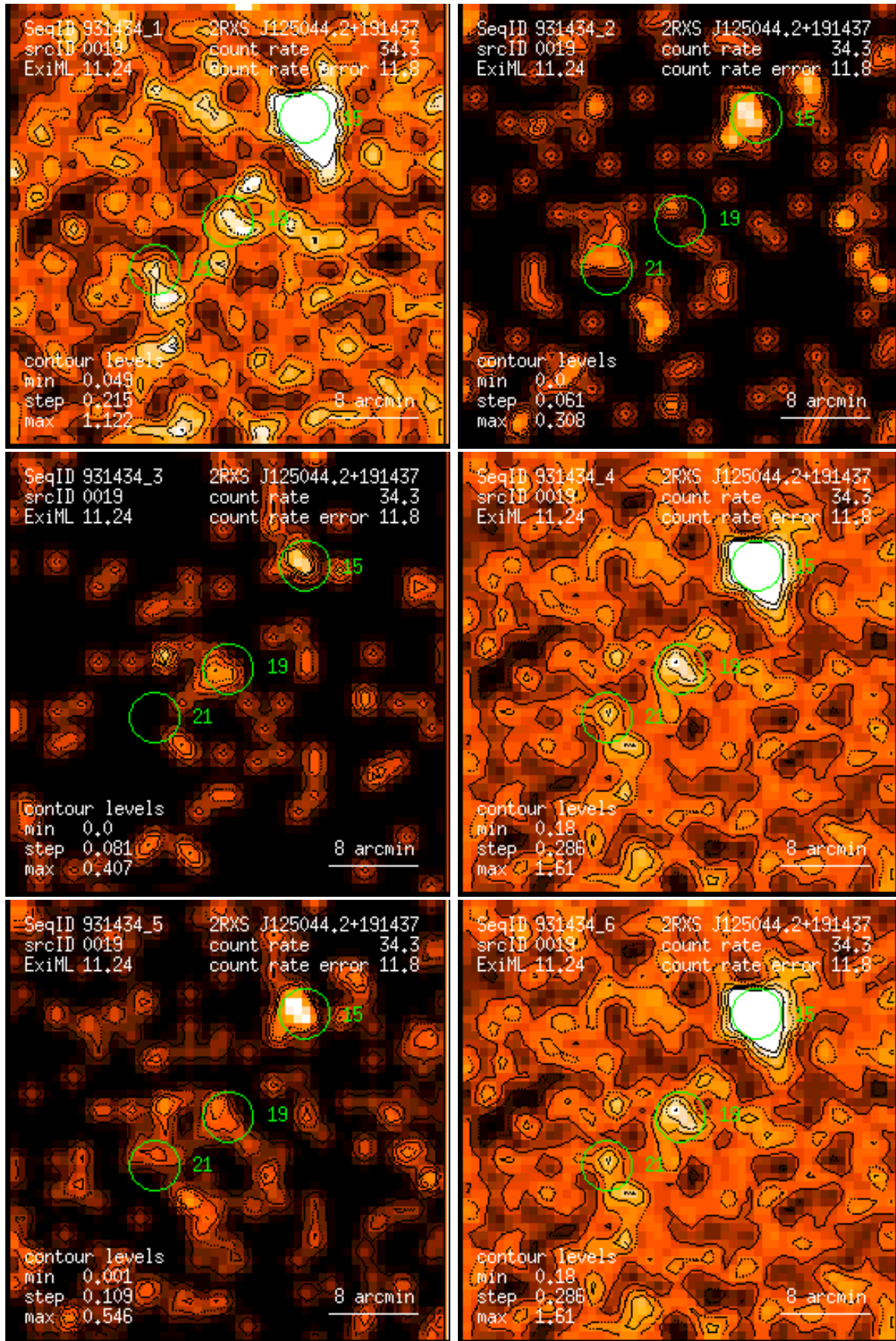
Figure 19: RASS 931434: detection 0019: band rate images, Gaussian filter: (1) PSPC channels 11 – 41, (2) 52 – 90, (3) 91 – 201, (4) 11 – 235, (5) 52 – 201, (6) 11 – 201. Broad band rates in counts/ks. Band rate contour levels in counts/ks/arcmin 2 .
