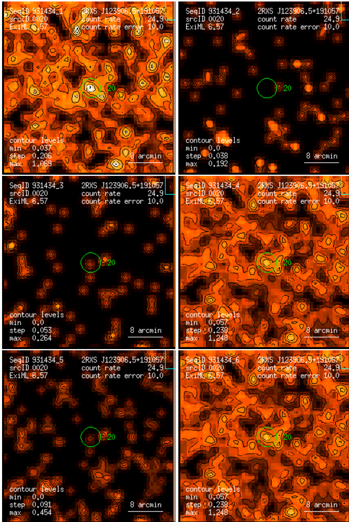
Figure 20: RASS 931434: detection 0020: band rate images, Gaussian filter: (1) PSPC channels 11 – 41, (2) 52 – 90, (3) 91 – 201, (4) 11 – 235, (5) 52 – 201, (6) 11 – 201. Broad band rates in counts/ks. Band rate contour levels in counts/ks/arcmin 2 .
