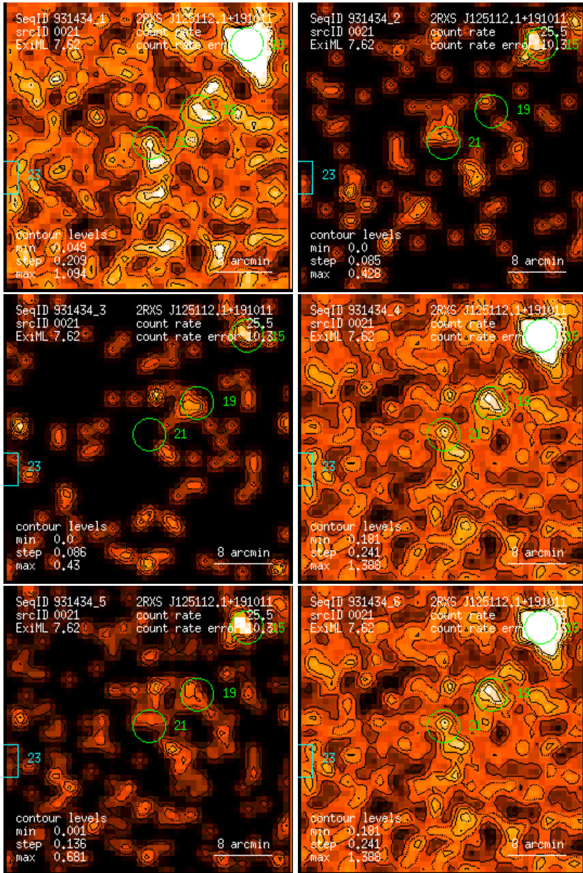
Figure 21: RASS 931434: detection 0021: band rate images, Gaussian filter: (1) PSPC channels 11 – 41, (2) 52 – 90, (3) 91 – 201, (4) 11 – 235, (5) 52 – 201, (6) 11 – 201. Broad band rates in counts/ks. Band rate contour levels in counts/ks/arcmin 2 .
