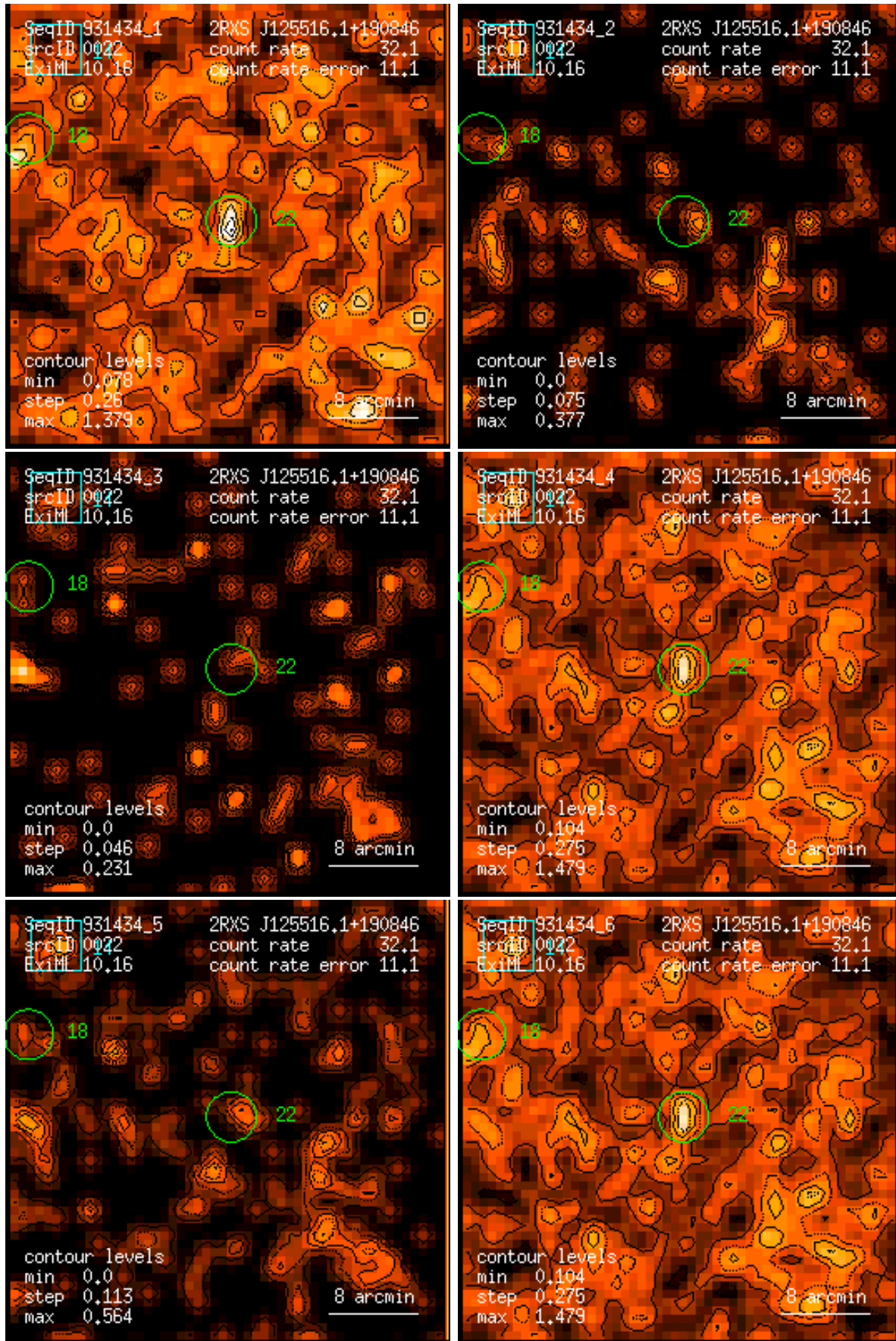
Figure 22: RASS 931434: detection 0022: band rate images, Gaussian filter: (1) PSPC channels 11 – 41, (2) 52 – 90, (3) 91 – 201, (4) 11 – 235, (5) 52 – 201, (6) 11 – 201. Broad band rates in counts/ks. Band rate contour levels in counts/ks/arcmin 2 .
