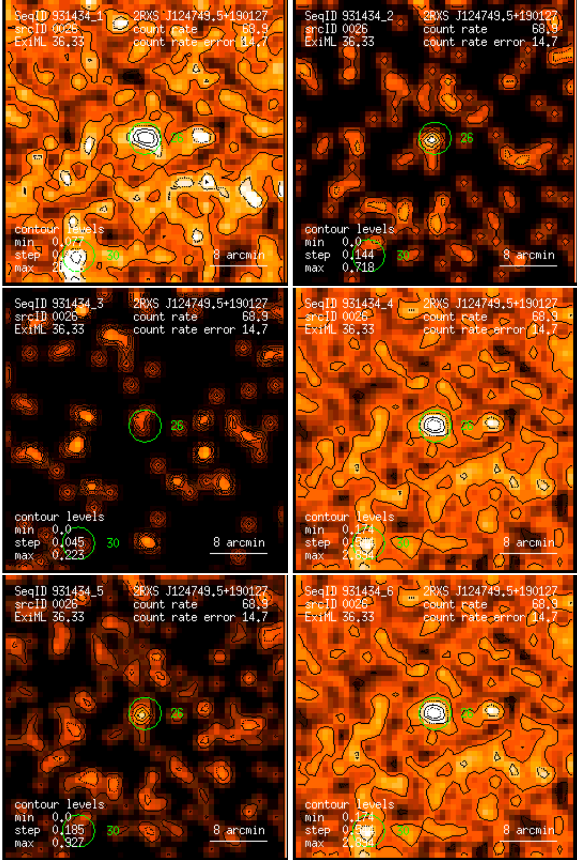
Figure 26: RASS 931434: detection 0026: band rate images, Gaussian filter: (1) PSPC channels 11 – 41, (2) 52 – 90, (3) 91 – 201, (4) 11 – 235, (5) 52 – 201, (6) 11 – 201. Broad band rates in counts/ks. Band rate contour levels in counts/ks/arcmin 2 .
