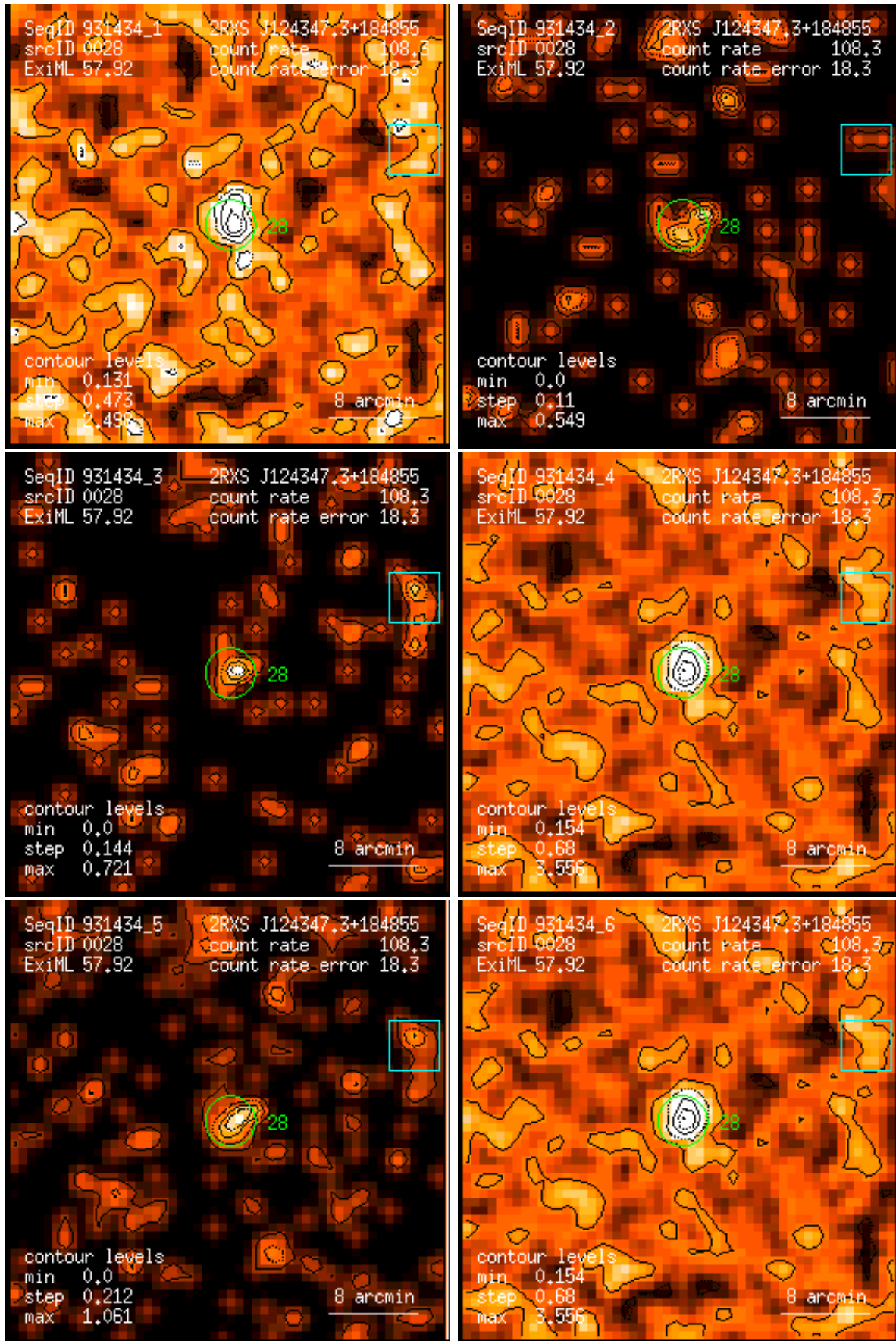
Figure 28: RASS 931434: detection 0028: band rate images, Gaussian filter: (1) PSPC channels 11 – 41, (2) 52 – 90, (3) 91 – 201, (4) 11 – 235, (5) 52 – 201, (6) 11 – 201. Broad band rates in counts/ks. Band rate contour levels in counts/ks/arcmin 2 .
