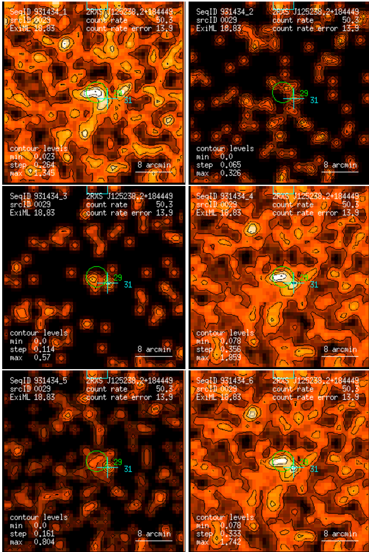
Figure 29: RASS 931434: detection 0029: band rate images, Gaussian filter: (1) PSPC channels 11 – 41, (2) 52 – 90, (3) 91 – 201, (4) 11 – 235, (5) 52 – 201, (6) 11 – 201. Broad band rates in counts/ks. Band rate contour levels in counts/ks/arcmin 2 .
