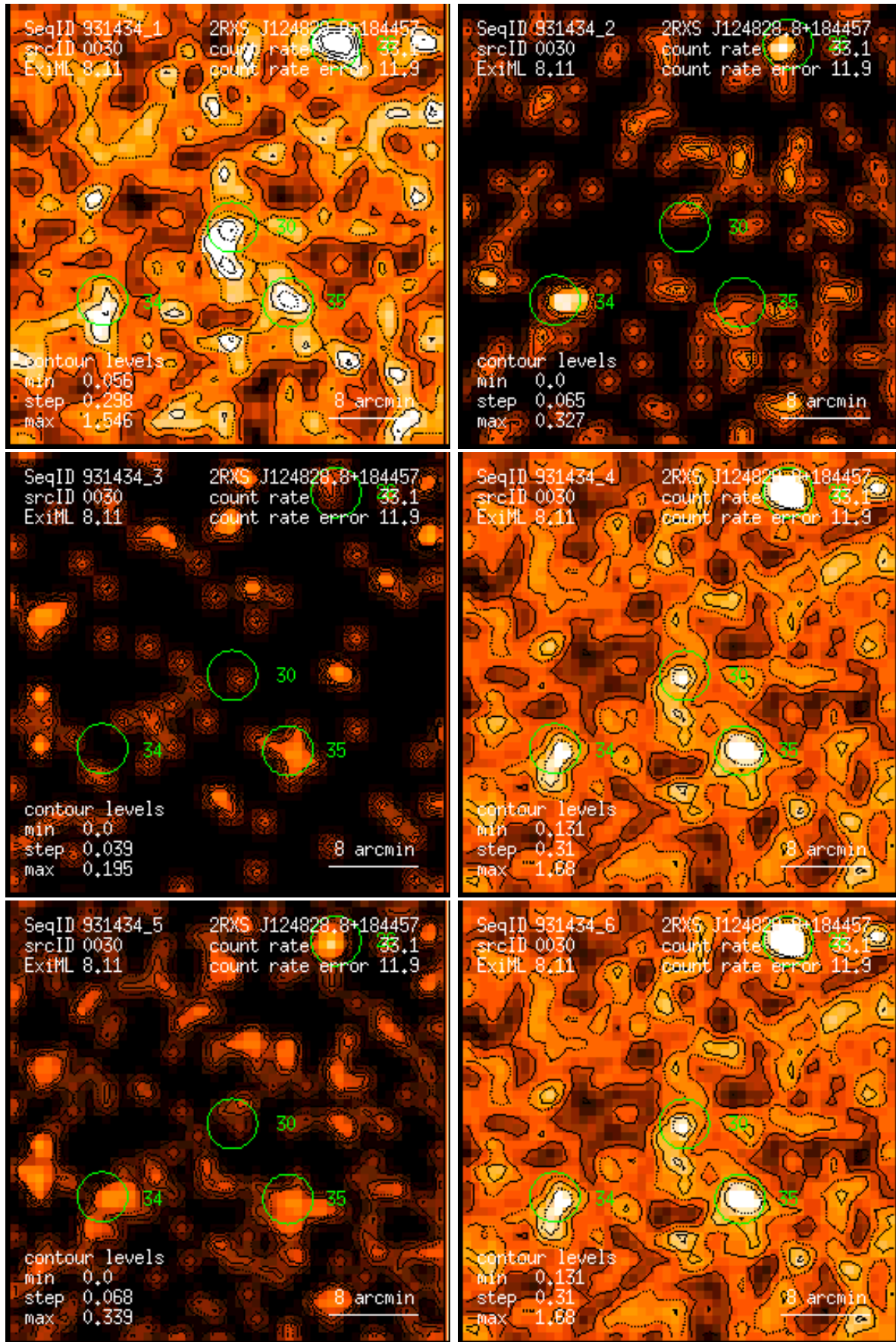
Figure 30: RASS 931434: detection 0030: band rate images, Gaussian filter: (1) PSPC channels 11 – 41, (2) 52 – 90, (3) 91 – 201, (4) 11 – 235, (5) 52 – 201, (6) 11 – 201. Broad band rates in counts/ks. Band rate contour levels in counts/ks/arcmin 2 .
