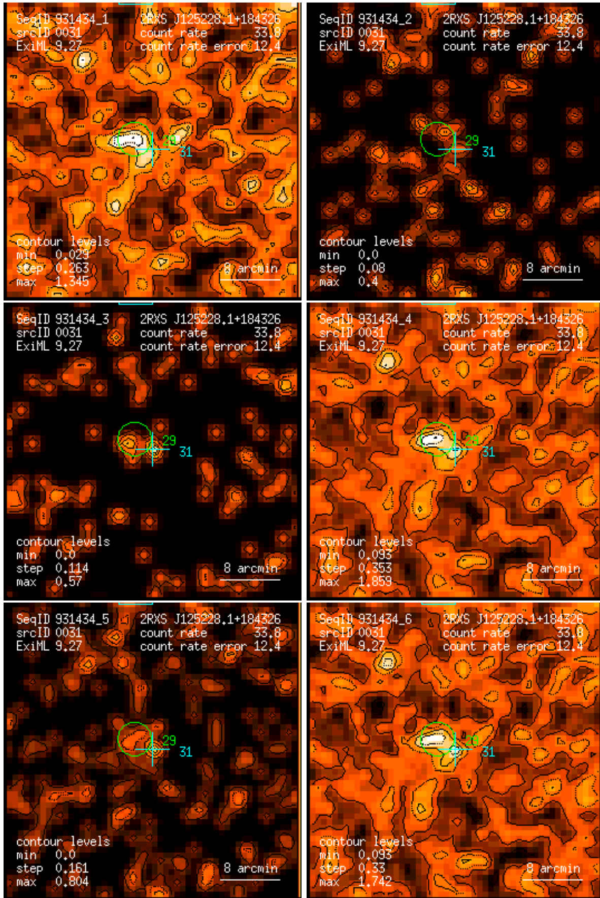
Figure 31: RASS 931434: detection 0031: band rate images, Gaussian filter: (1) PSPC channels 11 – 41, (2) 52 – 90, (3) 91 – 201, (4) 11 – 235, (5) 52 – 201, (6) 11 – 201. Broad band rates in counts/ks. Band rate contour levels in counts/ks/arcmin 2 .
