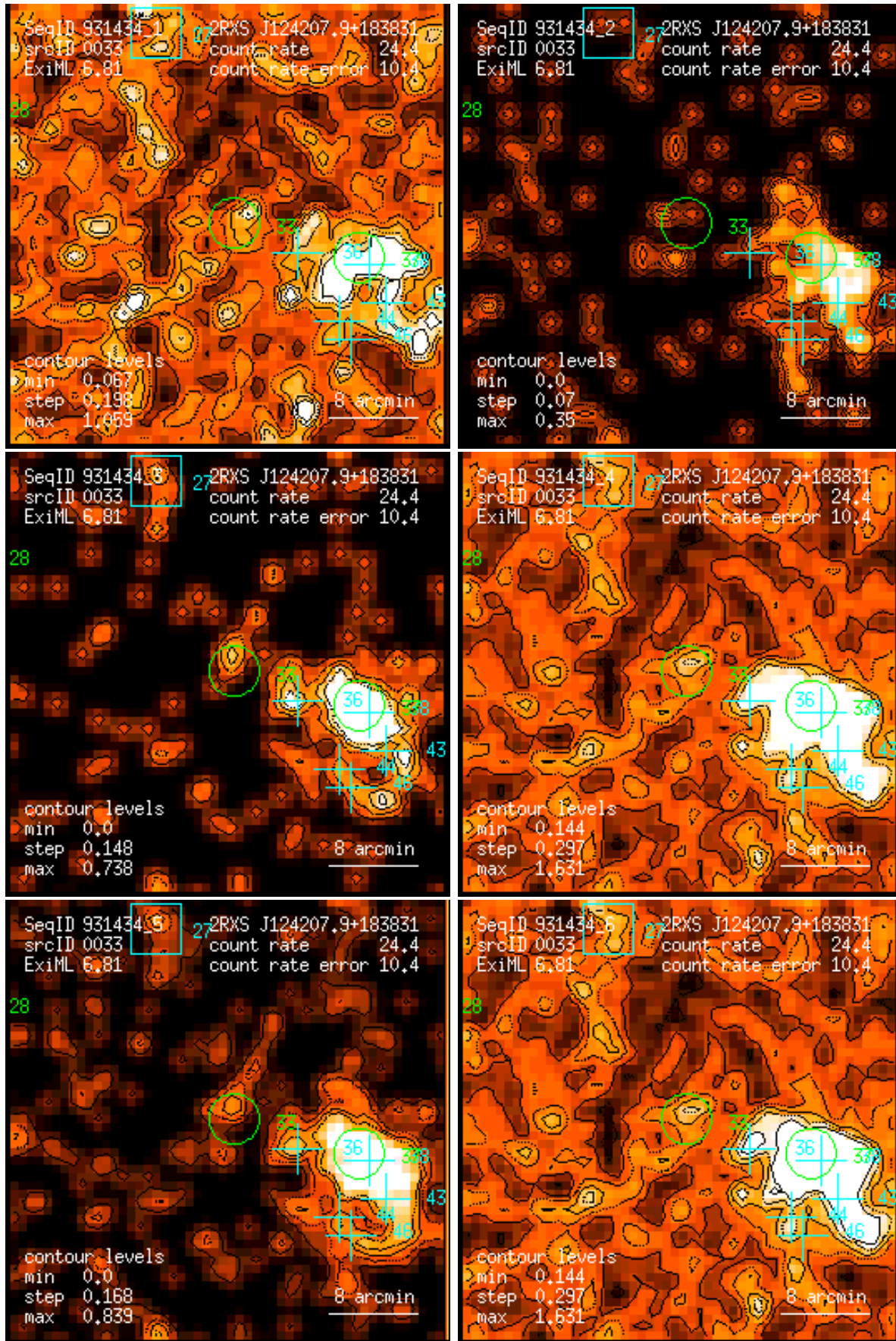
Figure 33: RASS 931434: detection 0033: band rate images, Gaussian filter: (1) PSPC channels 11 – 41, (2) 52 – 90, (3) 91 – 201, (4) 11 – 235, (5) 52 – 201, (6) 11 – 201. Broad band rates in counts/ks. Band rate contour levels in counts/ks/arcmin 2 .
