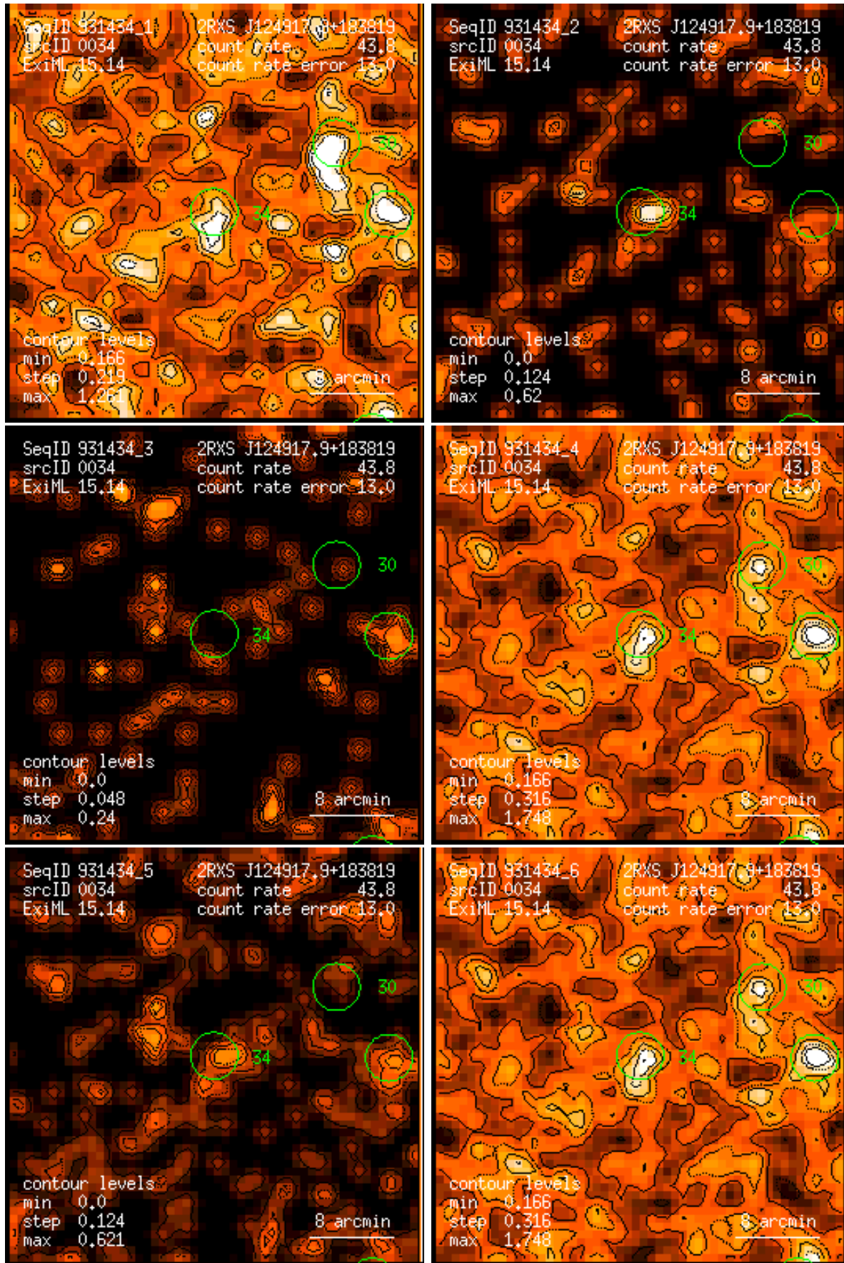
Figure 34: RASS 931434: detection 0034: band rate images, Gaussian filter: (1) PSPC channels 11 – 41, (2) 52 – 90, (3) 91 – 201, (4) 11 – 235, (5) 52 – 201, (6) 11 – 201. Broad band rates in counts/ks. Band rate contour levels in counts/ks/arcmin 2 .
